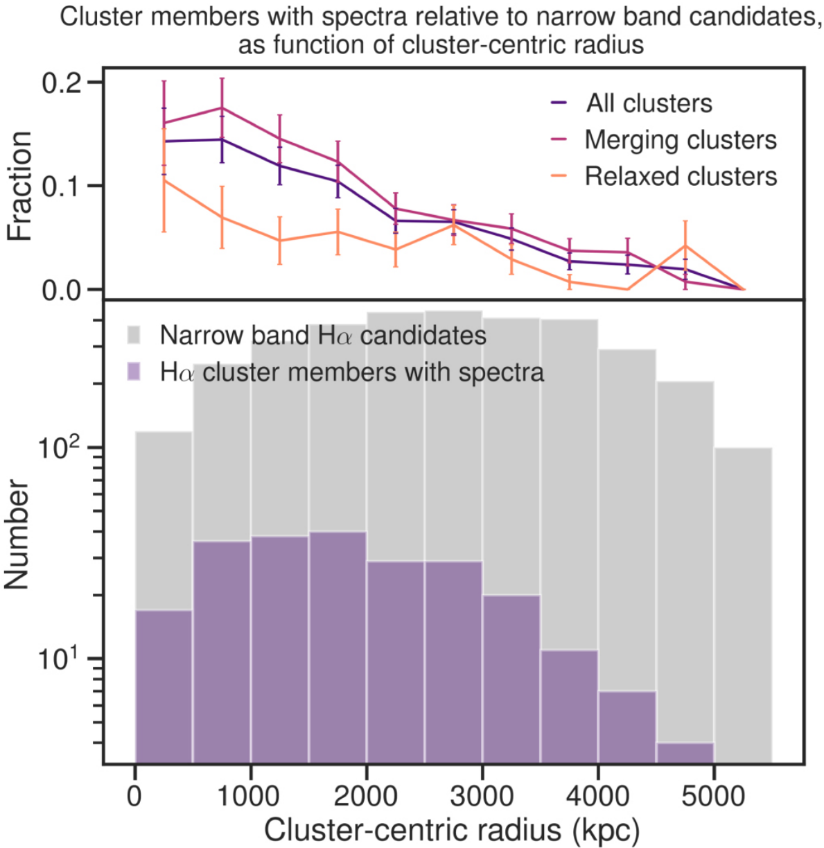
Figure 7. from ENISALA. II. Distinct Star Formation and Active Galactic Nucleus Activity in Merging and Relaxed Galaxy Clusters null 2021 APJ 912 55 doi:10.3847/1538-4357/abe7f8 https://dx.doi.org/10.3847/1538-4357/abe7f8 © 2021. The American Astronomical Society. All rights reserved.
