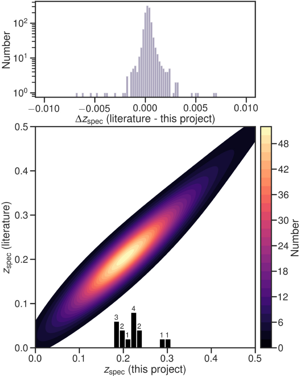
Figure 4. from ENISALA. II. Distinct Star Formation and Active Galactic Nucleus Activity in Merging and Relaxed Galaxy Clusters null 2021 APJ 912 55 doi:10.3847/1538-4357/abe7f8 https://dx.doi.org/10.3847/1538-4357/abe7f8 © 2021. The American Astronomical Society. All rights reserved.
