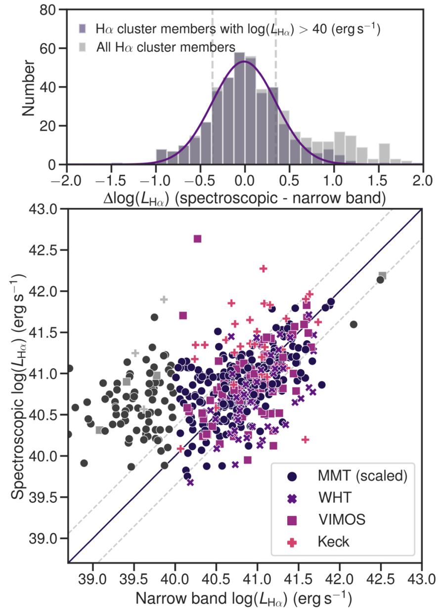
Figure 3. from ENISALA. II. Distinct Star Formation and Active Galactic Nucleus Activity in Merging and Relaxed Galaxy Clusters null 2021 APJ 912 55 doi:10.3847/1538-4357/abe7f8 https://dx.doi.org/10.3847/1538-4357/abe7f8
