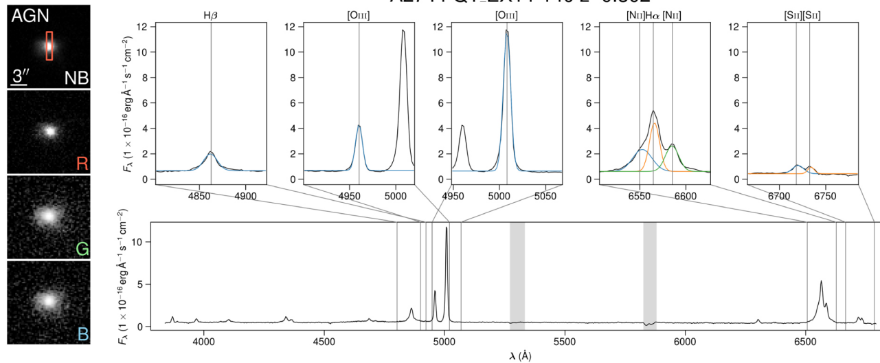
(b) AGN dominated spectrum taken with VLT/VIMOS.
