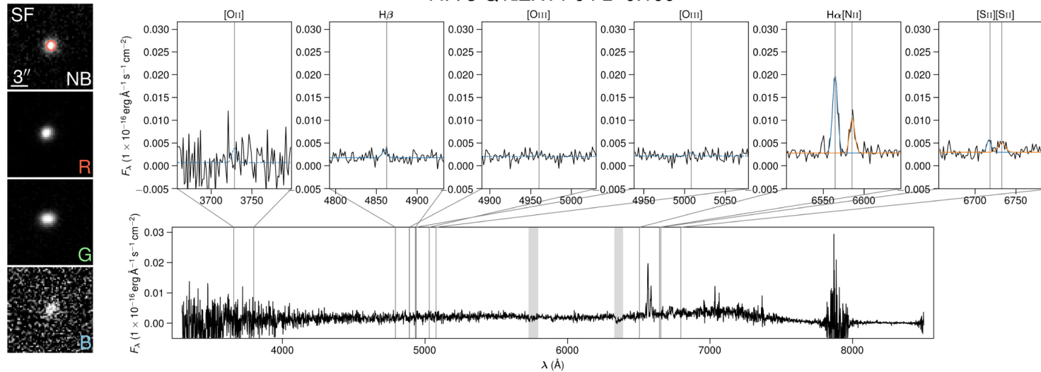
(a) SF dominated spectrum taken with WHT/AF2.
