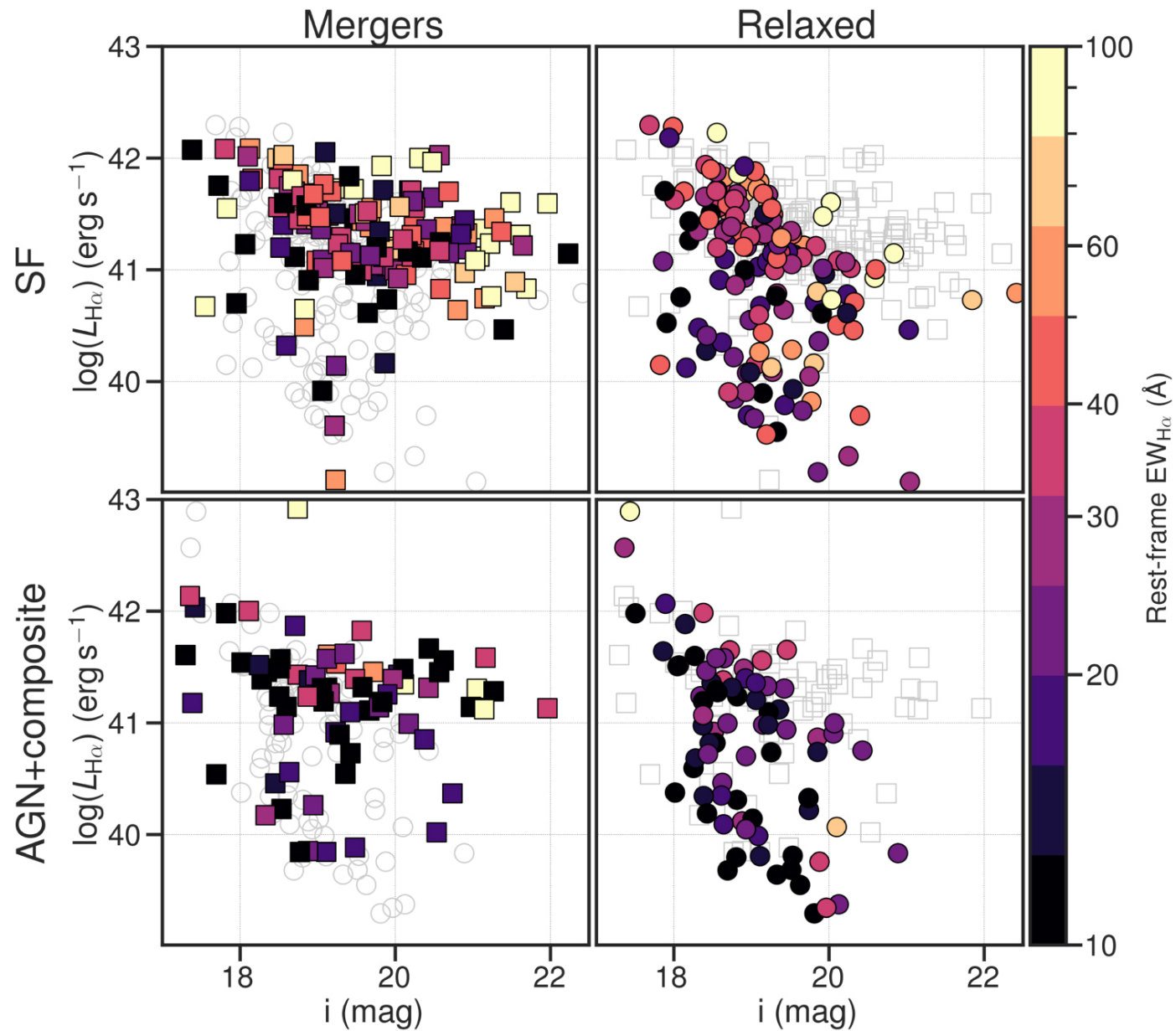
Figure 19. from ENISALA. II. Distinct Star Formation and Active Galactic Nucleus Activity in Merging and Relaxed Galaxy Clusters null 2021 APJ 912 55 doi:10.3847/1538-4357/abe7f8 https://dx.doi.org/10.3847/1538-4357/abe7f8 © 2021. The American Astronomical Society. All rights reserved.
