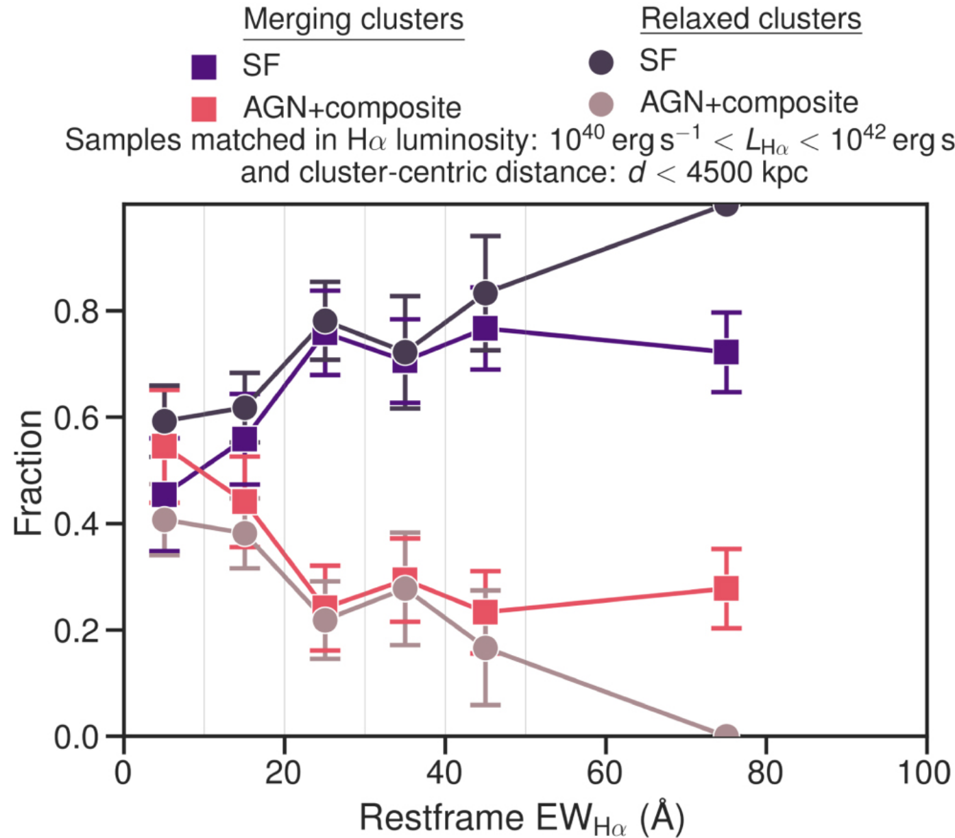
Figure 18. from ENISALA. II. Distinct Star Formation and Active Galactic Nucleus Activity in Merging and Relaxed Galaxy Clusters null 2021 APJ 912 55 doi:10.3847/1538-4357/abe7f8 https://dx.doi.org/10.3847/1538-4357/abe7f8 © 2021. The American Astronomical Society. All rights reserved.
