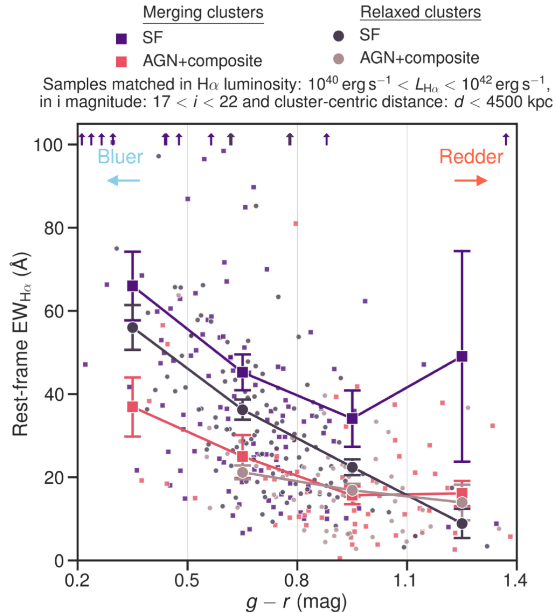
Figure 17. from ENISALA. II. Distinct Star Formation and Active Galactic Nucleus Activity in Merging and Relaxed Galaxy Clusters null 2021 APJ 912 55 doi:10.3847/1538-4357/abe7f8 https://dx.doi.org/10.3847/1538-4357/abe7f8 © 2021. The American Astronomical Society. All rights reserved.
