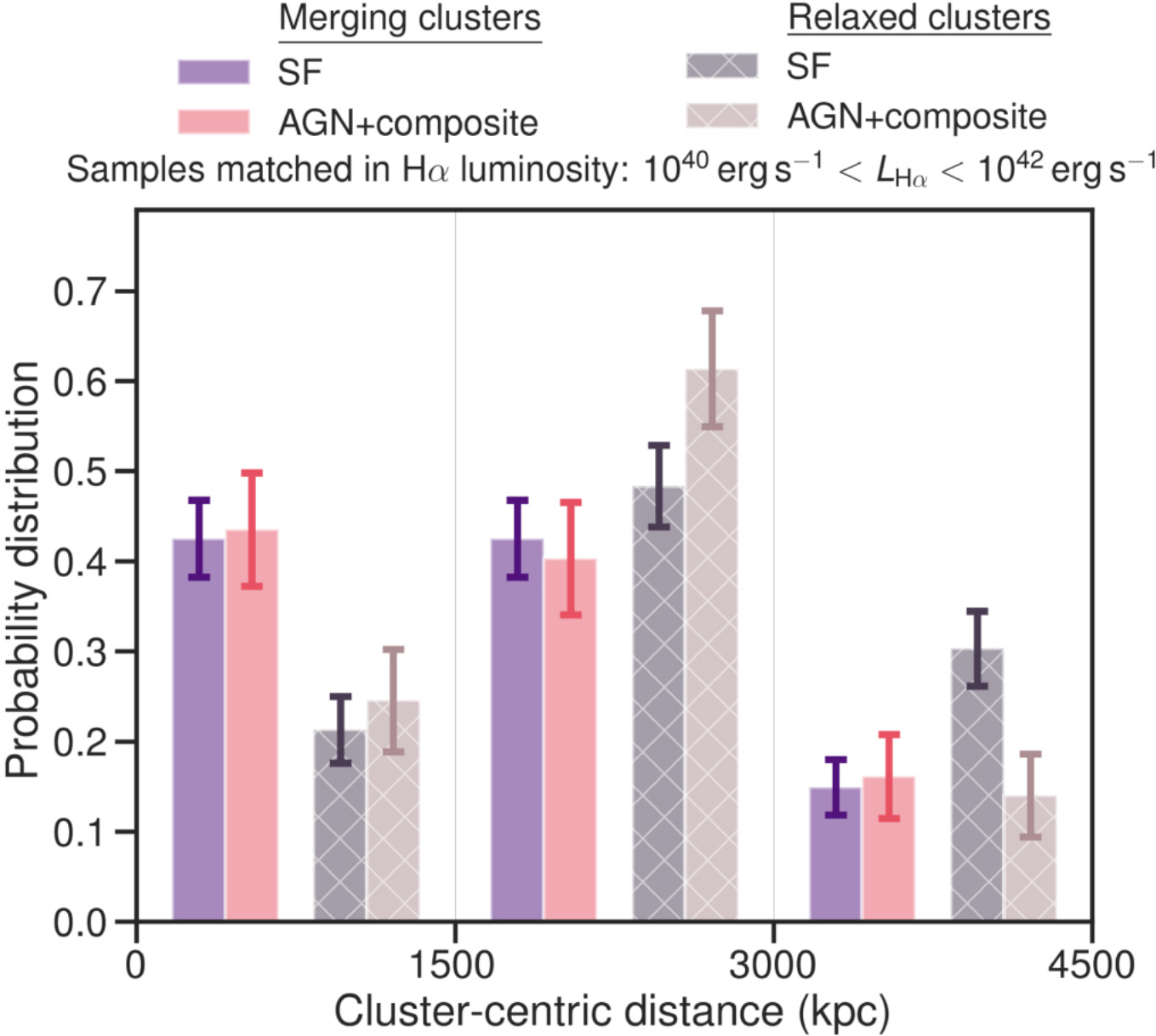
Figure 15. from ENISALA. II. Distinct Star Formation and Active Galactic Nucleus Activity in Merging and Relaxed Galaxy Clusters null 2021 APJ 912 55 doi:10.3847/1538-4357/abe7f8 https://dx.doi.org/10.3847/1538-4357/abe7f8 © 2021. The American Astronomical Society. All rights reserved.
