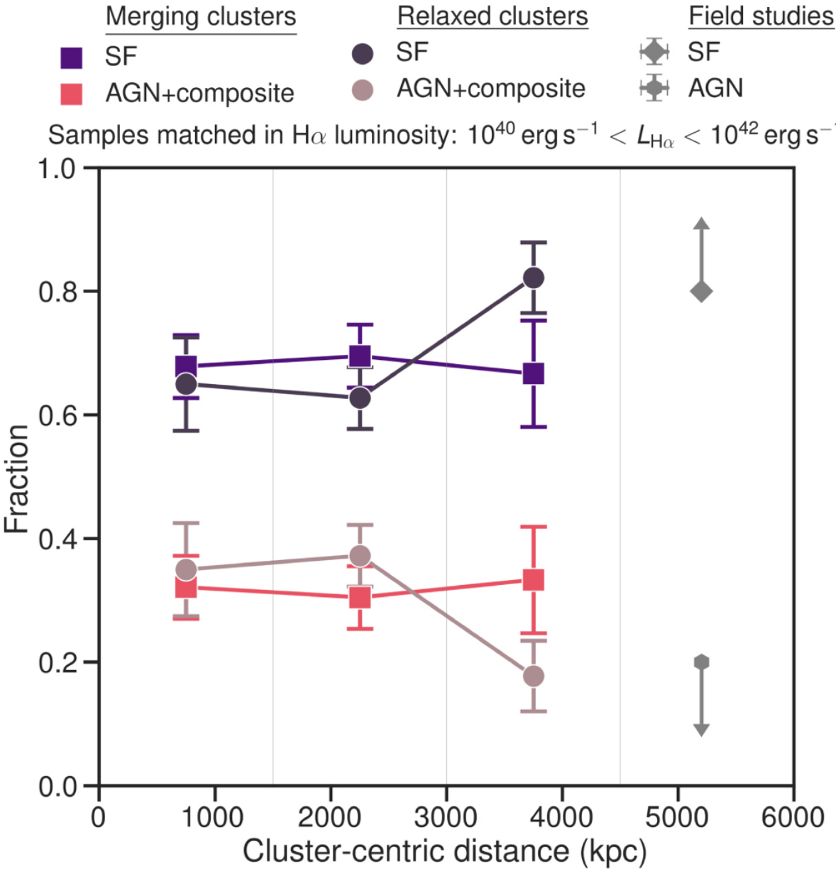
Figure 14. from ENISALA. II. Distinct Star Formation and Active Galactic Nucleus Activity in Merging and Relaxed Galaxy Clusters null 2021 APJ 912 55 doi:10.3847/1538-4357/abe7f8 https://dx.doi.org/10.3847/1538-4357/abe7f8 © 2021. The American Astronomical Society. All rights reserved.
