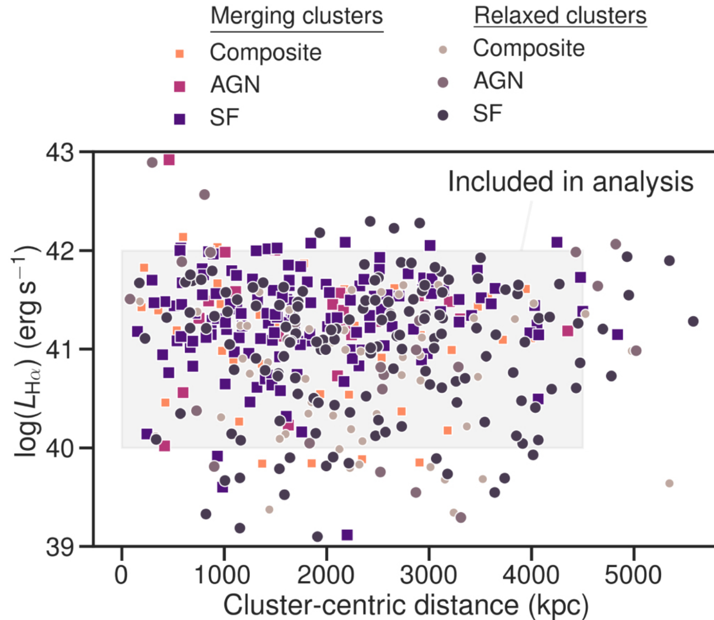
Figure 13. from ENISALA. II. Distinct Star Formation and Active Galactic Nucleus Activity in Merging and Relaxed Galaxy Clusters null 2021 APJ 912 55 doi:10.3847/1538-4357/abe7f8 https://dx.doi.org/10.3847/1538-4357/abe7f8 © 2021. The American Astronomical Society. All rights reserved.
