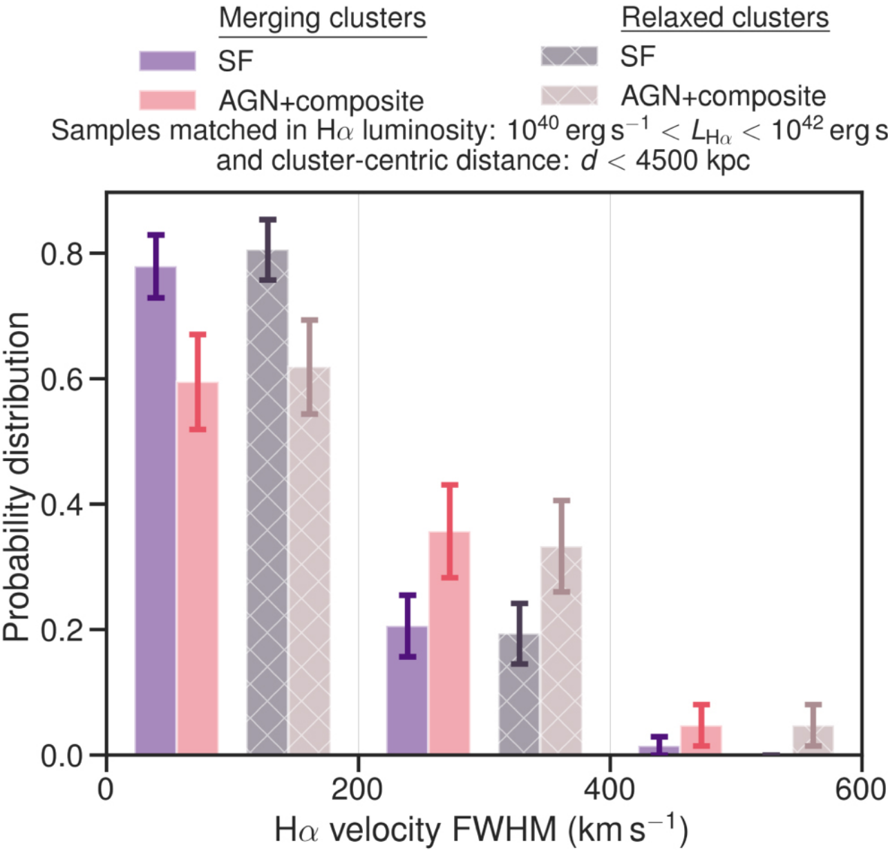
Figure 12. from ENISALA. II. Distinct Star Formation and Active Galactic Nucleus Activity in Merging and Relaxed Galaxy Clusters null 2021 APJ 912 55 doi:10.3847/1538-4357/abe7f8 https://dx.doi.org/10.3847/1538-4357/abe7f8 © 2021. The American Astronomical Society. All rights reserved.
