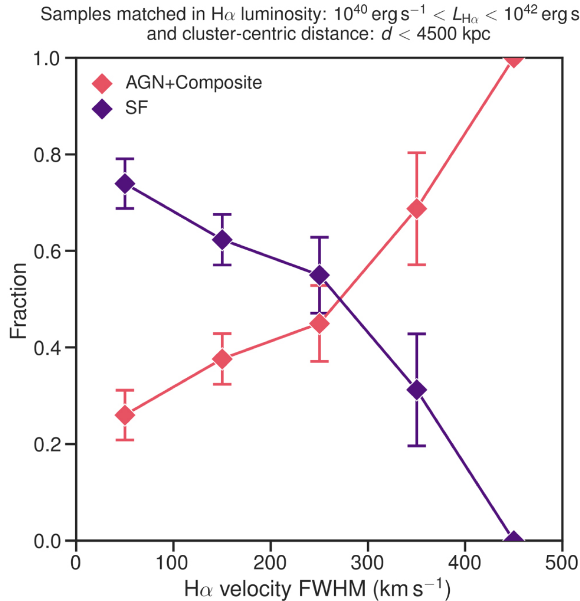
Figure 11. from ENISALA. II. Distinct Star Formation and Active Galactic Nucleus Activity in Merging and Relaxed Galaxy Clusters null 2021 APJ 912 55 doi:10.3847/1538-4357/abe7f8 https://dx.doi.org/10.3847/1538-4357/abe7f8 © 2021. The American Astronomical Society. All rights reserved.
