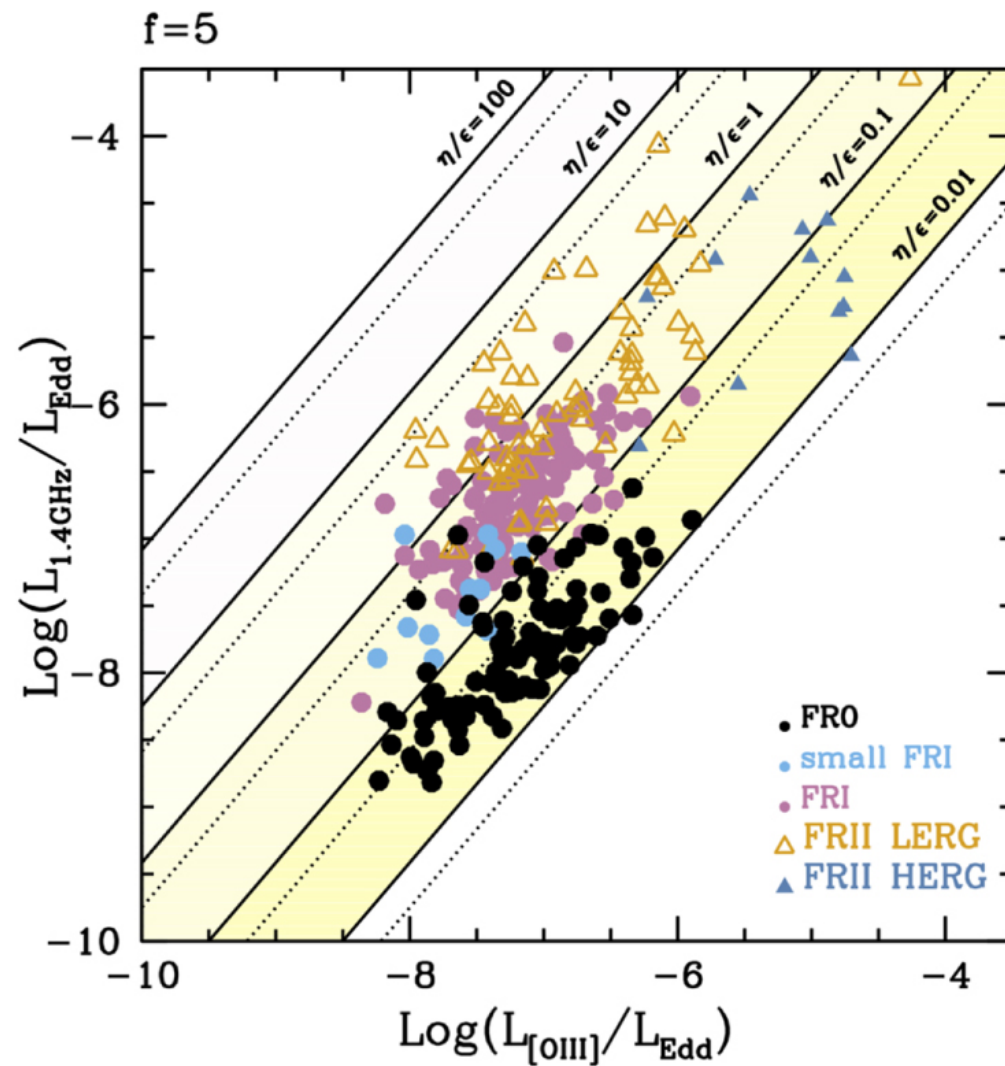
Figure 4. from Jet–Accretion System in the Nearby mJy Radio Galaxies null 2021 APJ 911 17 doi:10.3847/1538-4357/abe776 https://dx.doi.org/10.3847/1538-4357/abe776 © 2021. The Author(s). Published by the American Astronomical Society.
