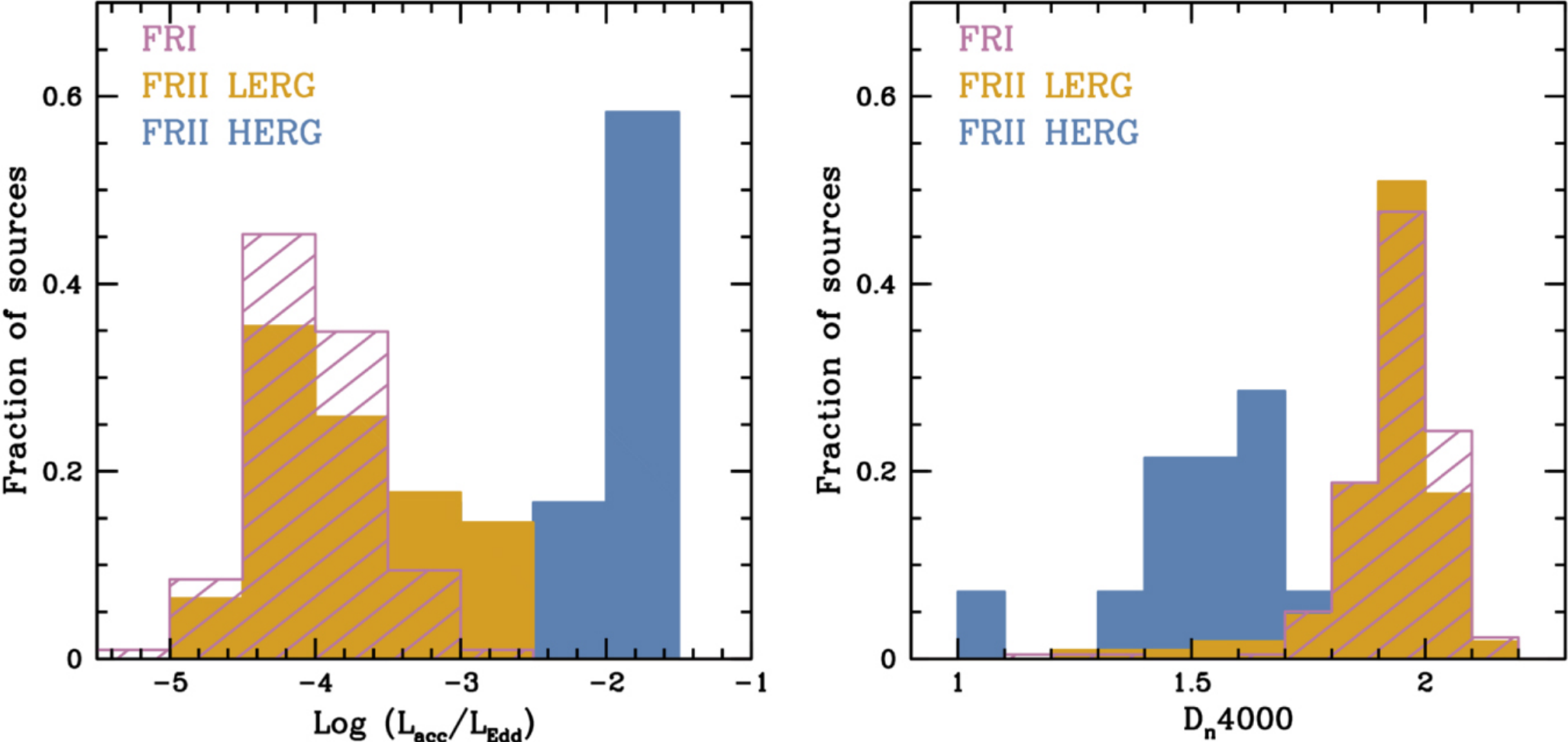
Figure 3. from Jet–Accretion System in the Nearby mJy Radio Galaxies null 2021 APJ 911 17 doi:10.3847/1538-4357/abe776 https://dx.doi.org/10.3847/1538-4357/abe776 © 2021. The Author(s). Published by the American Astronomical Society.
