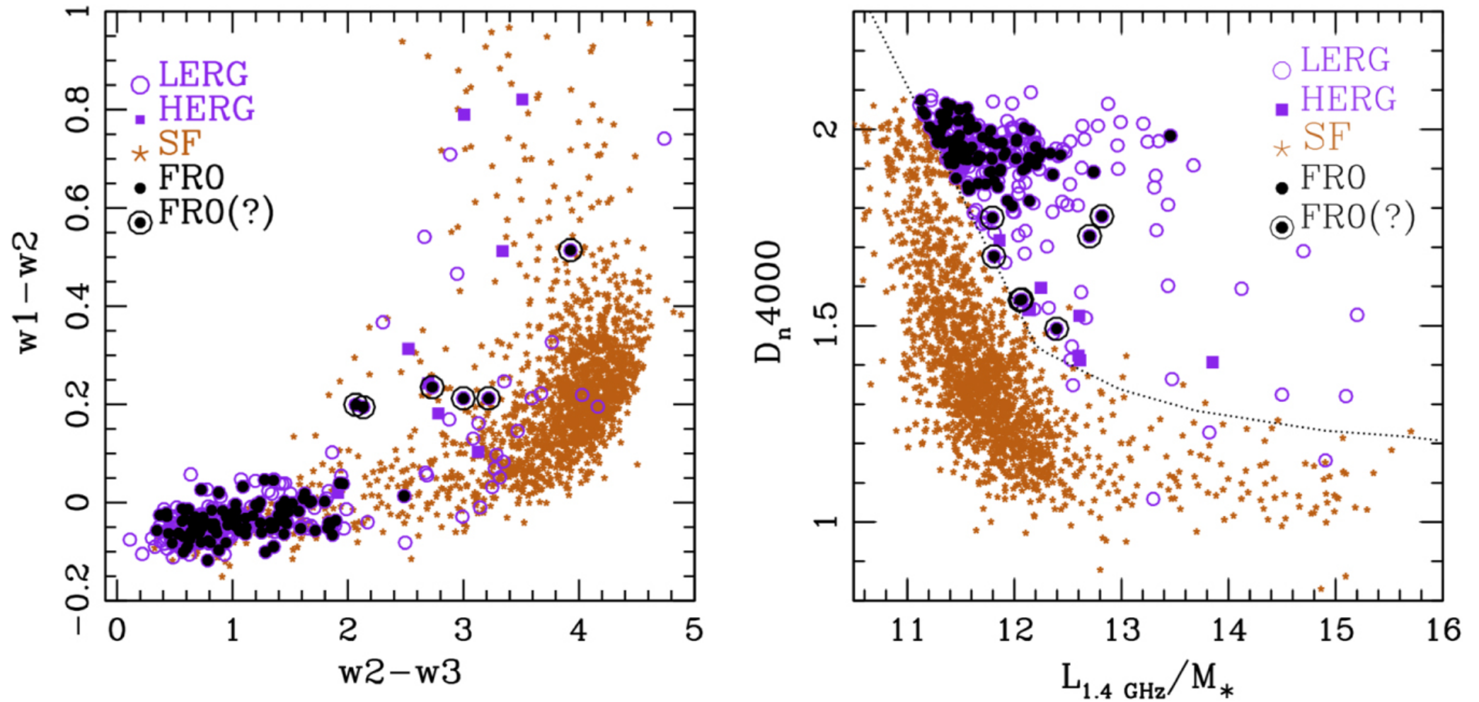
Figure 2. from Jet–Accretion System in the Nearby mJy Radio Galaxies null 2021 APJ 911 17 doi:10.3847/1538-4357/abe776 https://dx.doi.org/10.3847/1538-4357/abe776 © 2021. The Author(s). Published by the American Astronomical Society.
