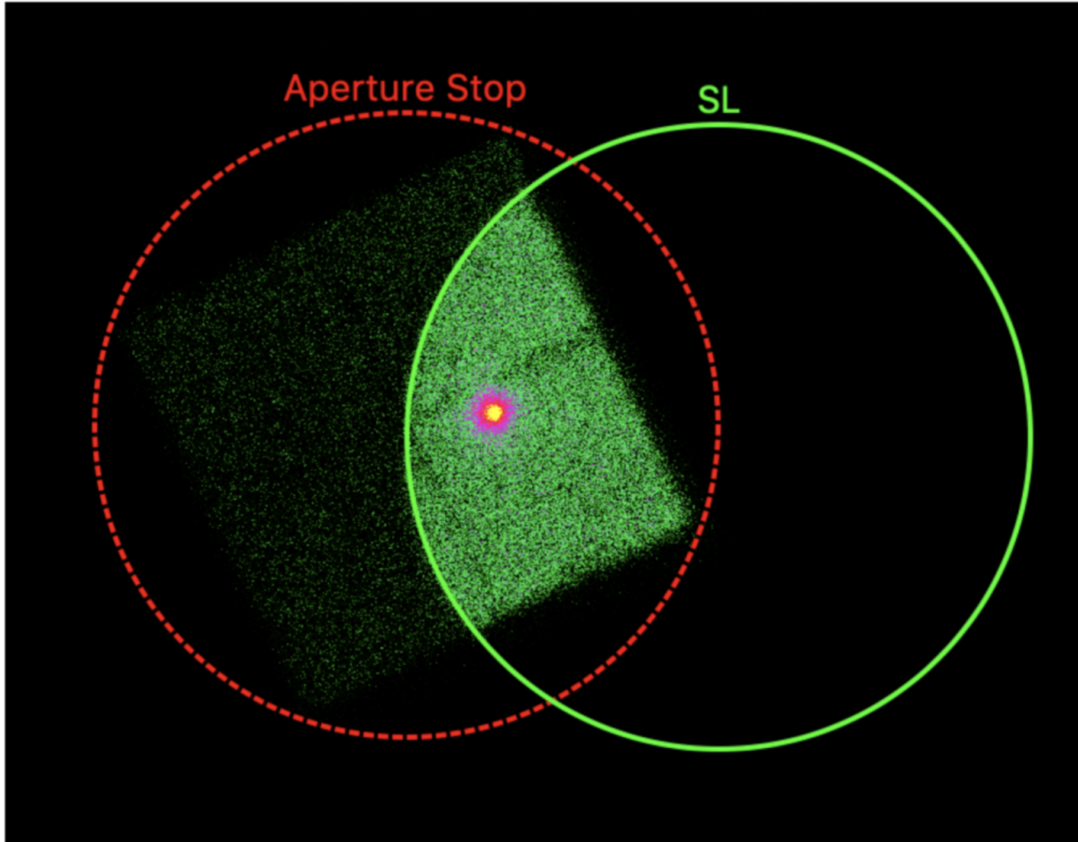
Figure 4. from StrayCats: A Catalog of NuSTAR Stray Light Observations null 2021 APJ 909 30 doi:10.3847/1538-4357/abe045 https://dx.doi.org/10.3847/1538-4357/abe045 © 2021. The American Astronomical Society. All rights reserved.
