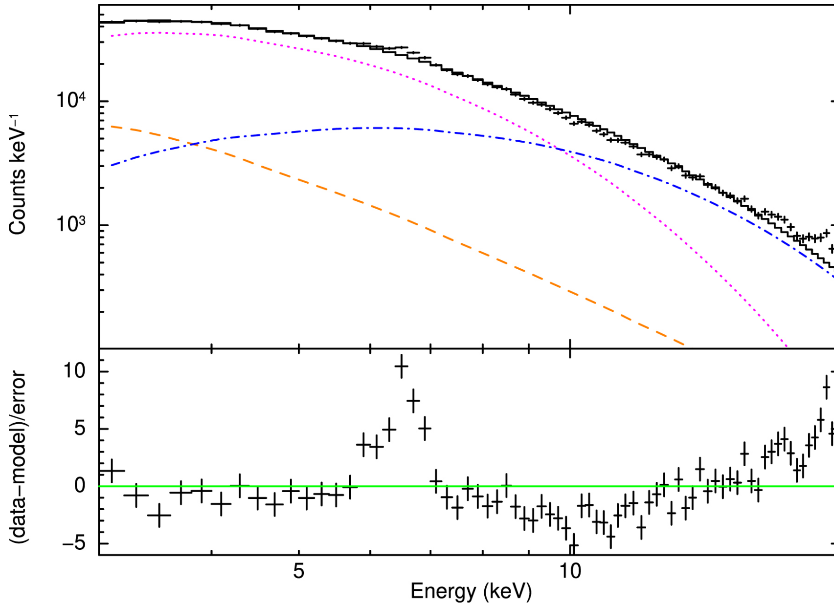
Figure 12. from StrayCats: A Catalog of NuSTAR Stray Light Observations null 2021 APJ 909 30 doi:10.3847/1538-4357/abe045 https://dx.doi.org/10.3847/1538-4357/abe045 © 2021. The American Astronomical Society. All rights reserved.
