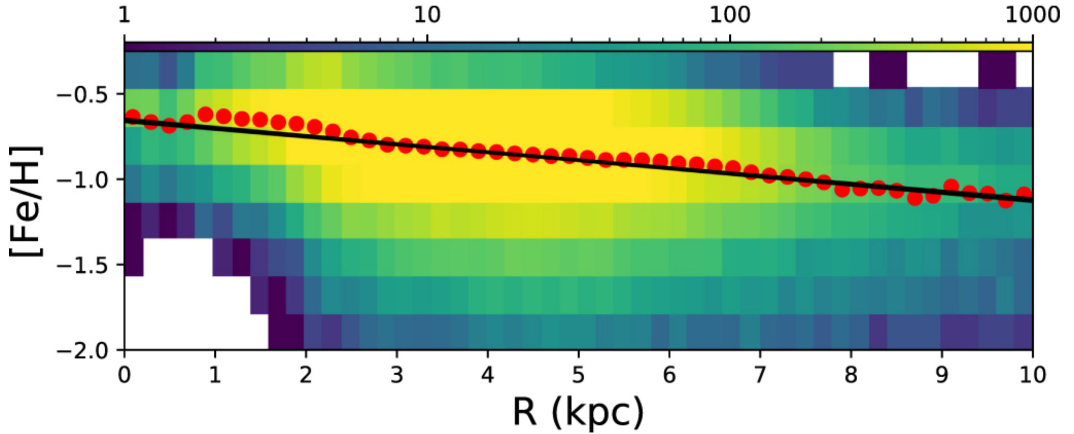
Figure 10. from Magellanic Mayhem: Metallicities and Motions null 2021 APJ 909 150 doi:10.3847/1538-4357/abd4e4 https://dx.doi.org/10.3847/1538-4357/abd4e4 © 2021. The American Astronomical Society. All rights reserved.
