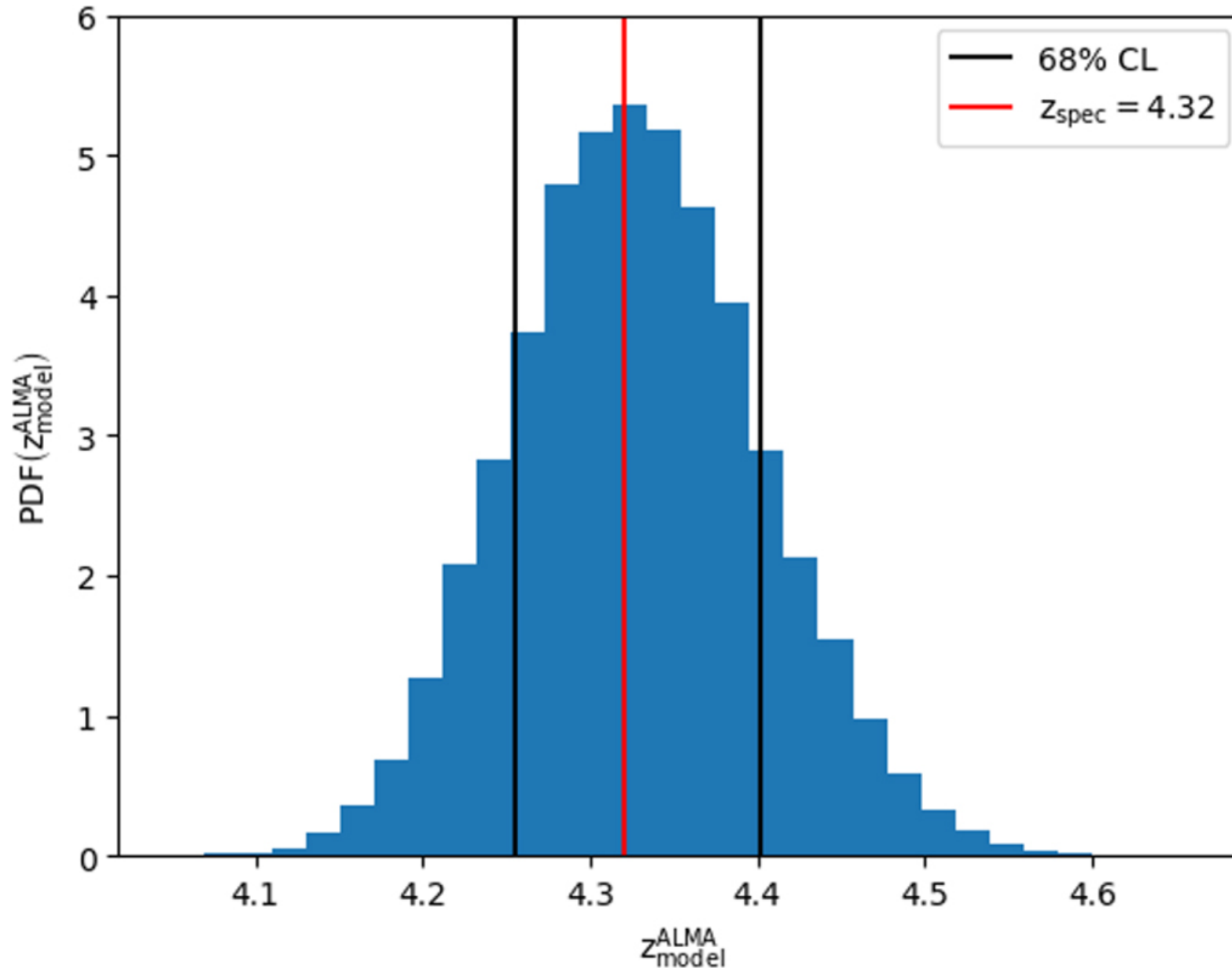
Figure 4. from ALMA Lensing Cluster Survey: An ALMA Galaxy Signposting a MUSE Galaxy Group at z = 4.3 Behind “El Gordo” null 2021 APJ 908 146 doi:10.3847/1538-4357/abd4d0 https://dx.doi.org/10.3847/1538-4357/abd4d0 © 2021. The American Astronomical Society. All rights reserved.
