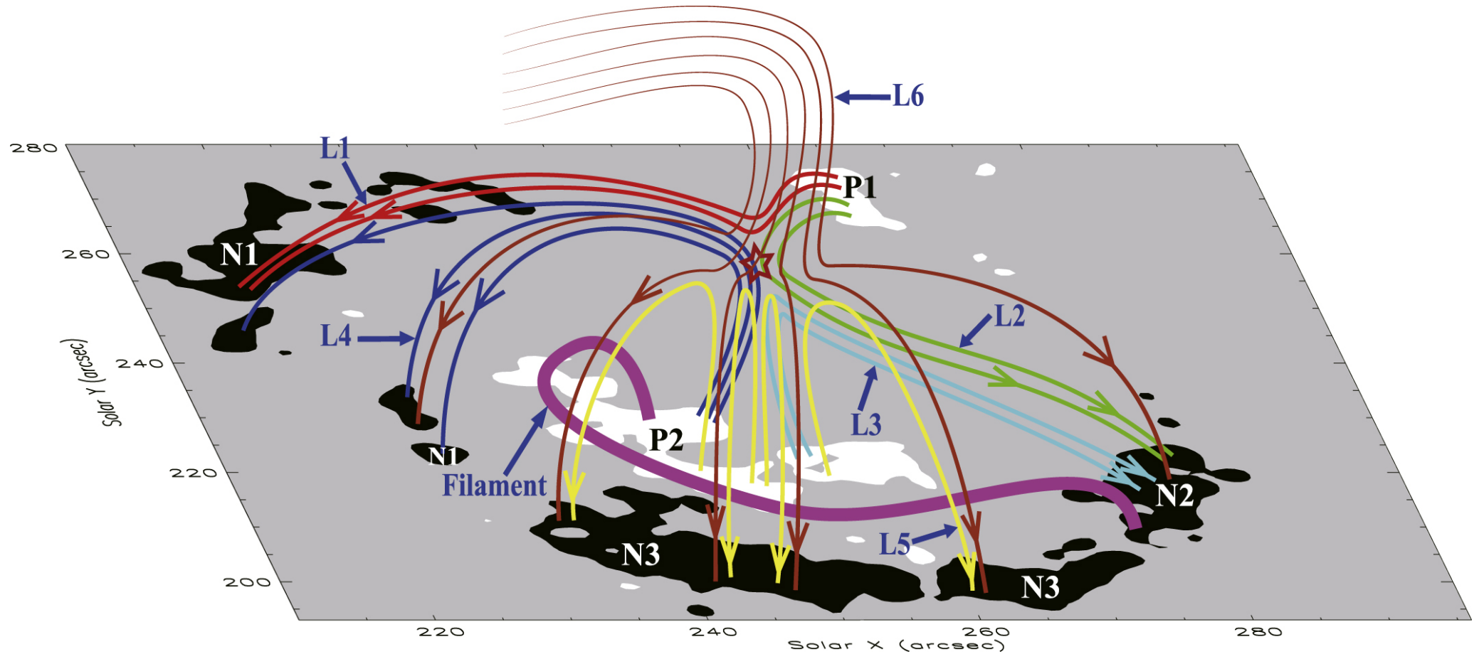
Figure 9. from Magnetic Reconnection between Loops Accelerated By a Nearby Filament Eruption null 2021 APJ 908 213 doi:10.3847/1538-4357/abd47e https://dx.doi.org/10.3847/1538-4357/abd47e © 2021. The American Astronomical Society. All rights reserved.
