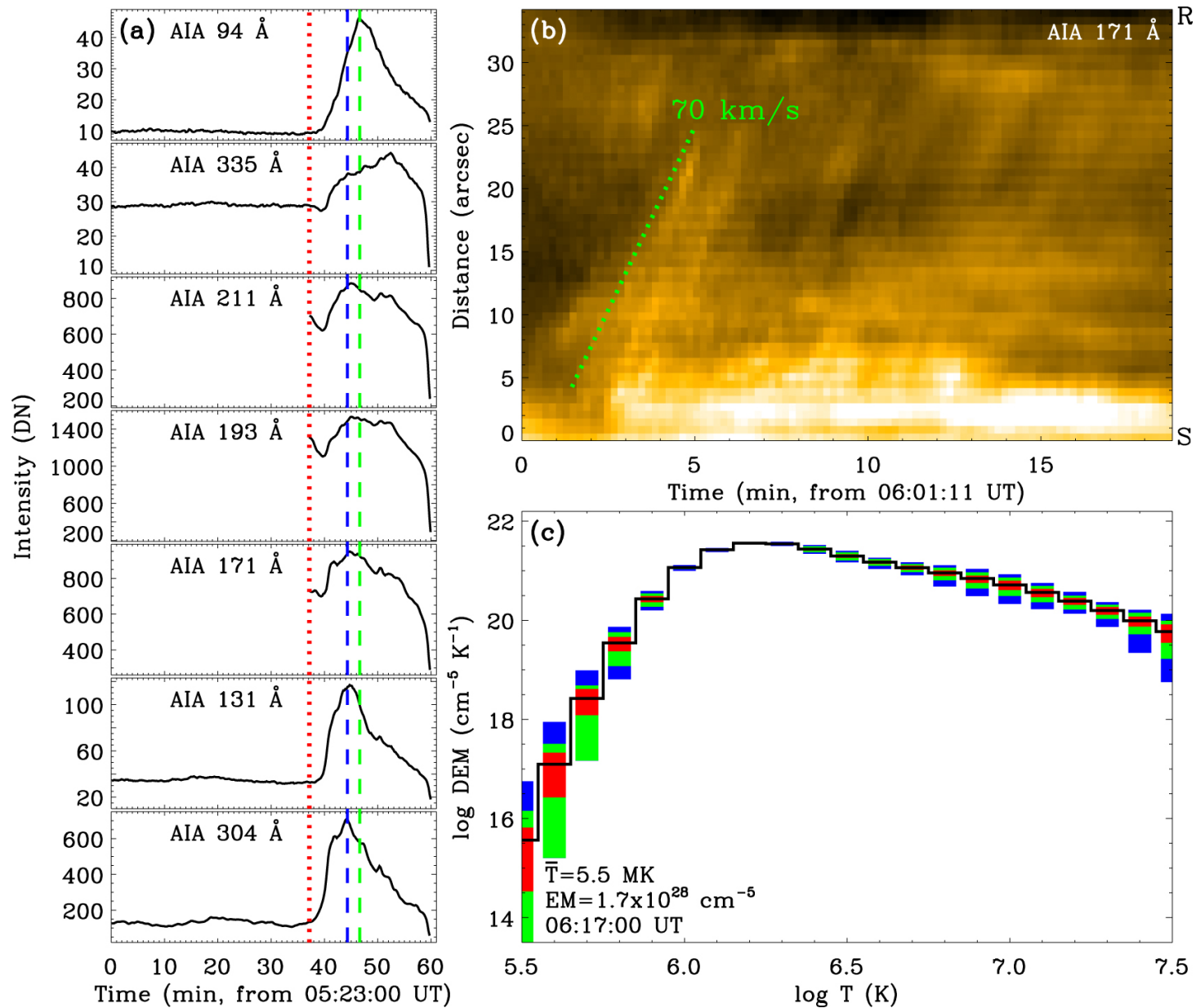
Figure 8. from Magnetic Reconnection between Loops Accelerated By a Nearby Filament Eruption null 2021 APJ 908 213 doi:10.3847/1538-4357/abd47e https://dx.doi.org/10.3847/1538-4357/abd47e © 2021. The American Astronomical Society. All rights reserved.
