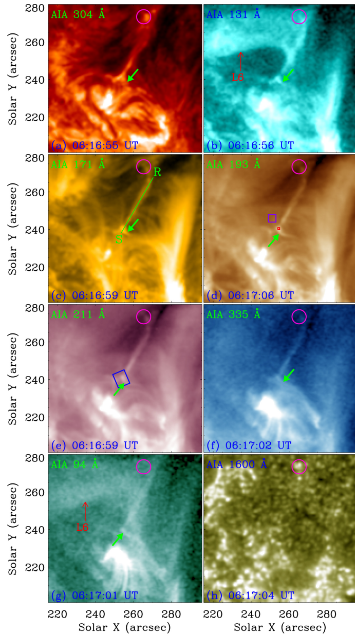
Figure 7. from Magnetic Reconnection between Loops Accelerated By a Nearby Filament Eruption null 2021 APJ 908 213 doi:10.3847/1538-4357/abd47e https://dx.doi.org/10.3847/1538-4357/abd47e
