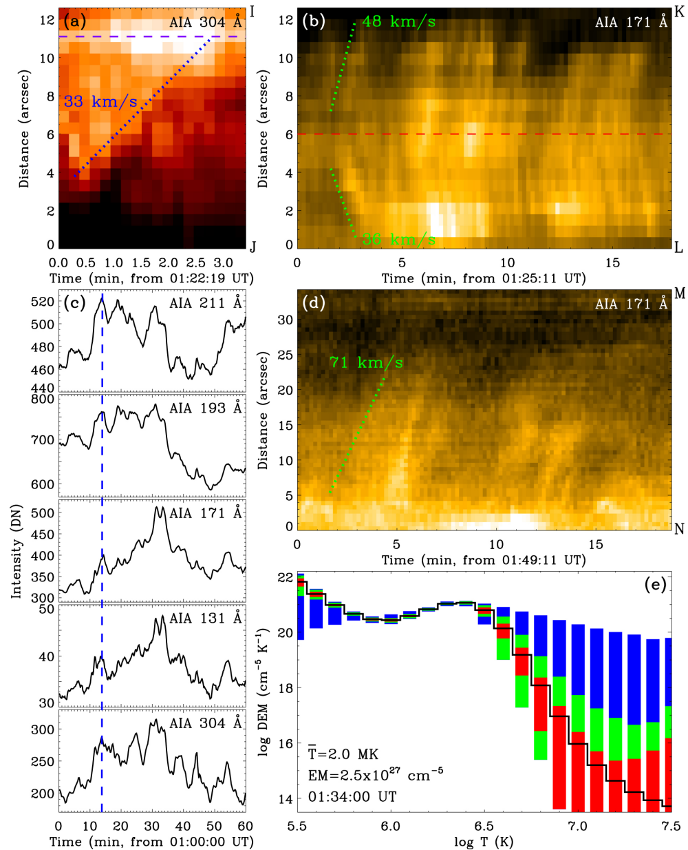
Figure 5. from Magnetic Reconnection between Loops Accelerated By a Nearby Filament Eruption null 2021 APJ 908 213 doi:10.3847/1538-4357/abd47e https://dx.doi.org/10.3847/1538-4357/abd47e © 2021. The American Astronomical Society. All rights reserved.
