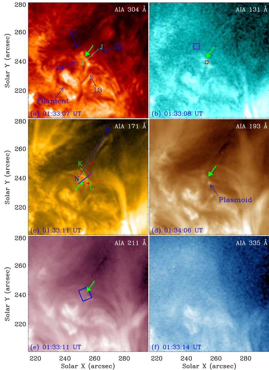
Figure 4. from Magnetic Reconnection between Loops Accelerated By a Nearby Filament Eruption null 2021 APJ 908 213 doi:10.3847/1538-4357/abd47e https://dx.doi.org/10.3847/1538-4357/abd47e
