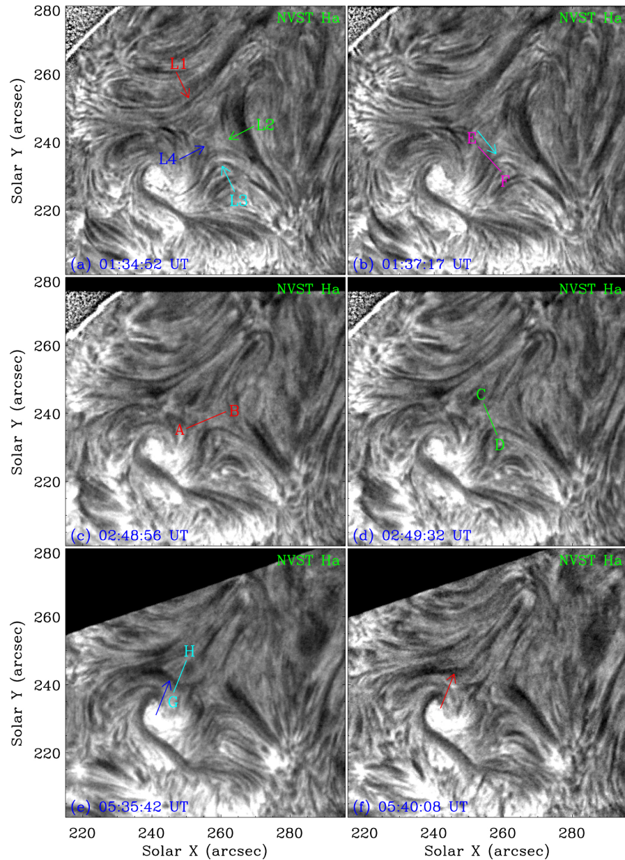
Figure 2. from Magnetic Reconnection between Loops Accelerated By a Nearby Filament Eruption null 2021 APJ 908 213 doi:10.3847/1538-4357/abd47e https://dx.doi.org/10.3847/1538-4357/abd47e
