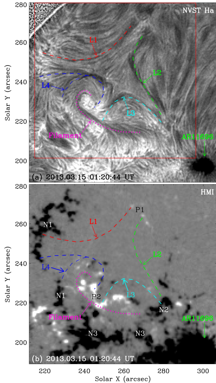
Figure 1. from Magnetic Reconnection between Loops Accelerated By a Nearby Filament Eruption null 2021 APJ 908 213 doi:10.3847/1538-4357/abd47e https://dx.doi.org/10.3847/1538-4357/abd47e
