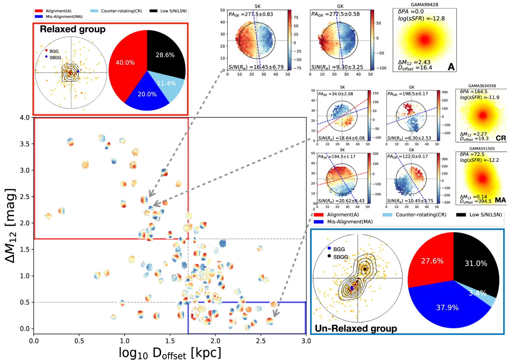
Figure 6. from The SAMI Galaxy Survey: Kinematics of Stars and Gas in Brightest Group Galaxies—The Role of Group Dynamics null 2021 APJ 908 123 doi:10.3847/1538-4357/abd47d https://dx.doi.org/10.3847/1538-4357/abd47d © 2021. The Author(s). Published by the American Astronomical Society.
