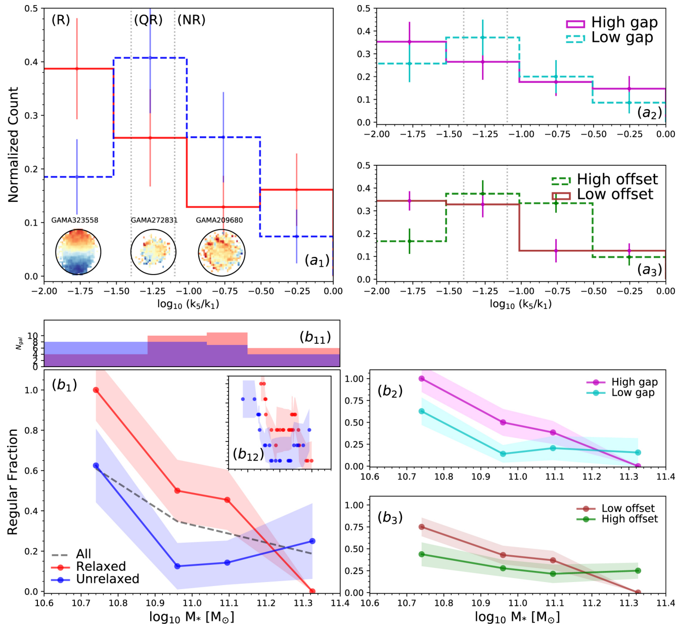
Figure 4. from The SAMI Galaxy Survey: Kinematics of Stars and Gas in Brightest Group Galaxies—The Role of Group Dynamics null 2021 APJ 908 123 doi:10.3847/1538-4357/abd47d https://dx.doi.org/10.3847/1538-4357/abd47d
