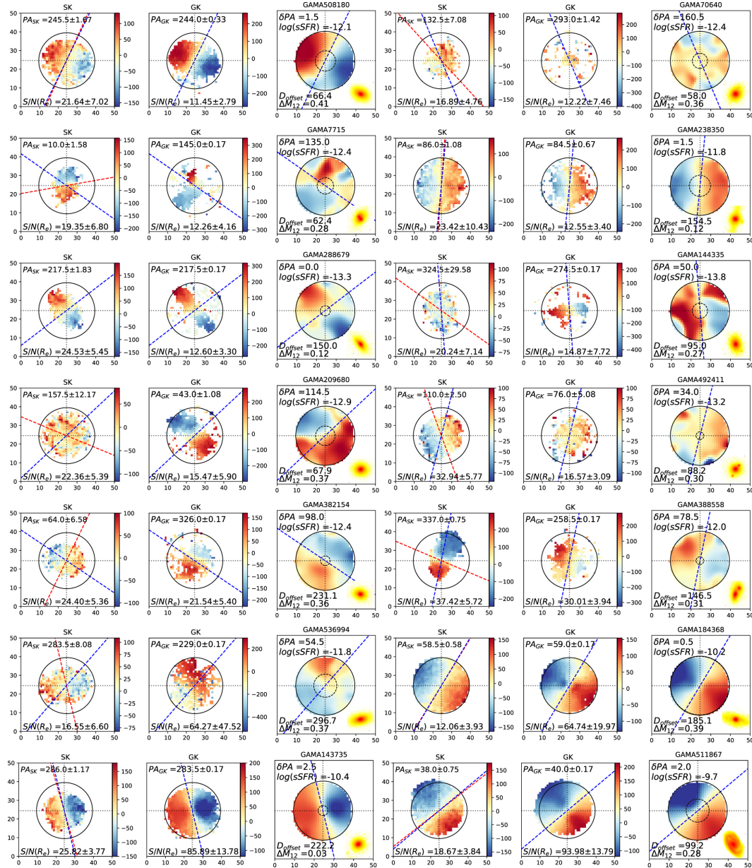
Figure 12. from The SAMI Galaxy Survey: Kinematics of Stars and Gas in Brightest Group Galaxies—The Role of Group Dynamics null 2021 APJ 908 123 doi:10.3847/1538-4357/abd47d https://dx.doi.org/10.3847/1538-4357/abd47d
