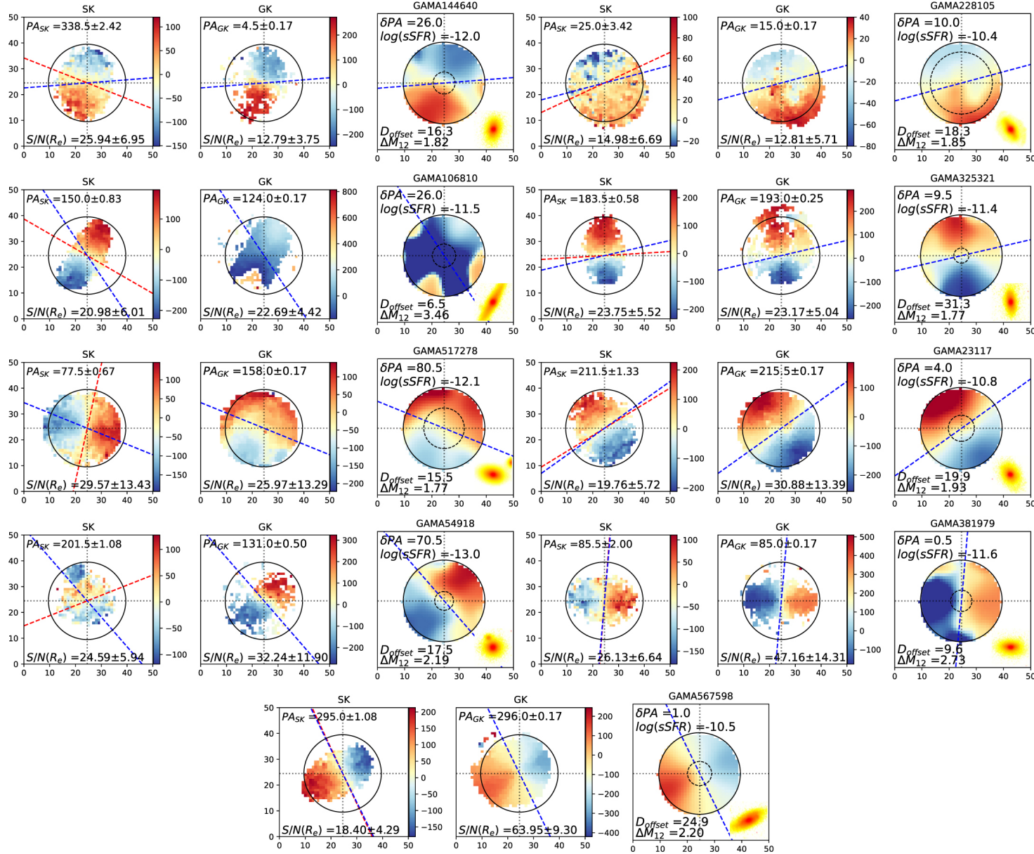
Figure 10. from The SAMI Galaxy Survey: Kinematics of Stars and Gas in Brightest Group Galaxies—The Role of Group Dynamics null 2021 APJ 908 123 doi:10.3847/1538-4357/abd47d https://dx.doi.org/10.3847/1538-4357/abd47d
