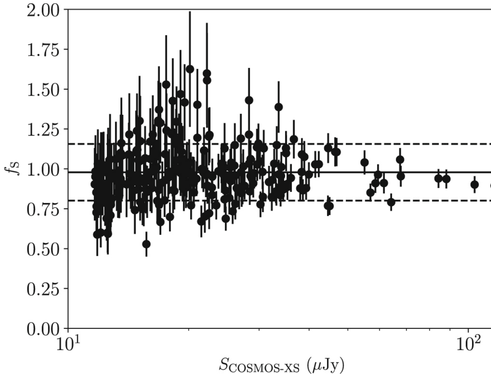
Figure 8. from An Ultradeep Multiband VLA Survey of the Faint Radio Sky (COSMOS-XS): Source Catalog and Number Counts null 2021 APJ 907 5 doi:10.3847/1538-4357/abcaa3 https://dx.doi.org/10.3847/1538-4357/abcaa3 © 2021. The American Astronomical Society. All rights reserved.
