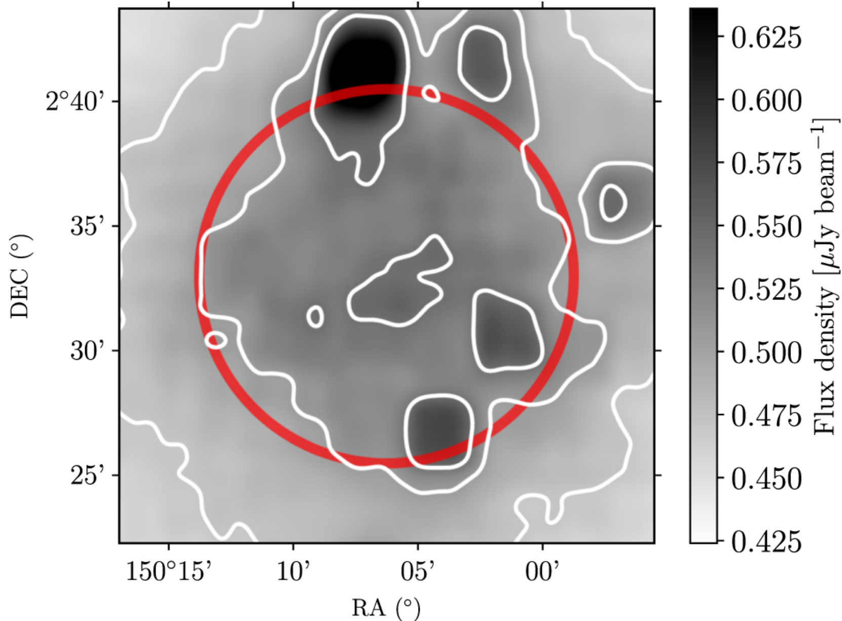
Figure 4. from An Ultradeep Multiband VLA Survey of the Faint Radio Sky (COSMOS-XS): Source Catalog and Number Counts null 2021 APJ 907 5 doi:10.3847/1538-4357/abcaa3 https://dx.doi.org/10.3847/1538-4357/abcaa3 © 2021. The American Astronomical Society. All rights reserved.
