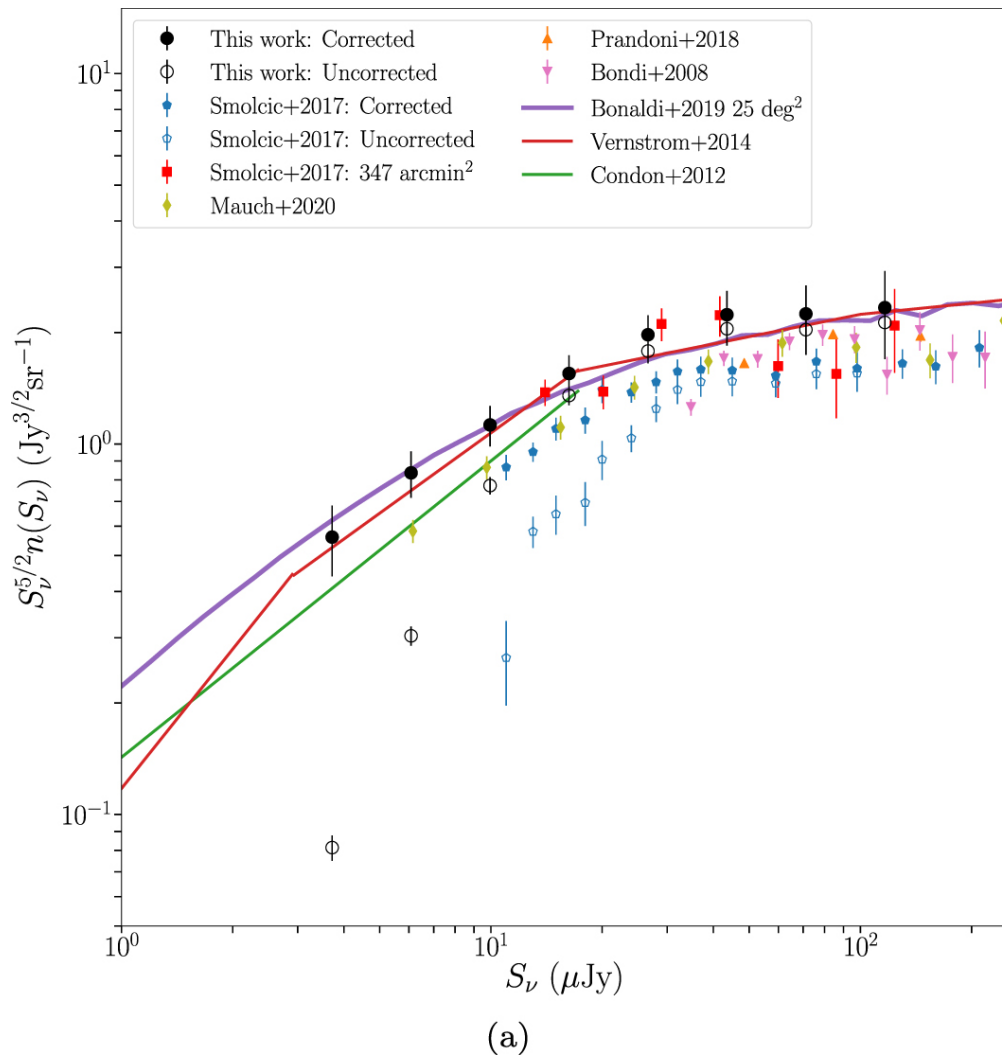
Figure 15. from An Ultradeep Multiband VLA Survey of the Faint Radio Sky (COSMOS-XS): Source Catalog and Number Counts null 2021 APJ 907 5 doi:10.3847/1538-4357/abcaa3 https://dx.doi.org/10.3847/1538-4357/abcaa3 © 2021. The American Astronomical Society. All rights reserved.
