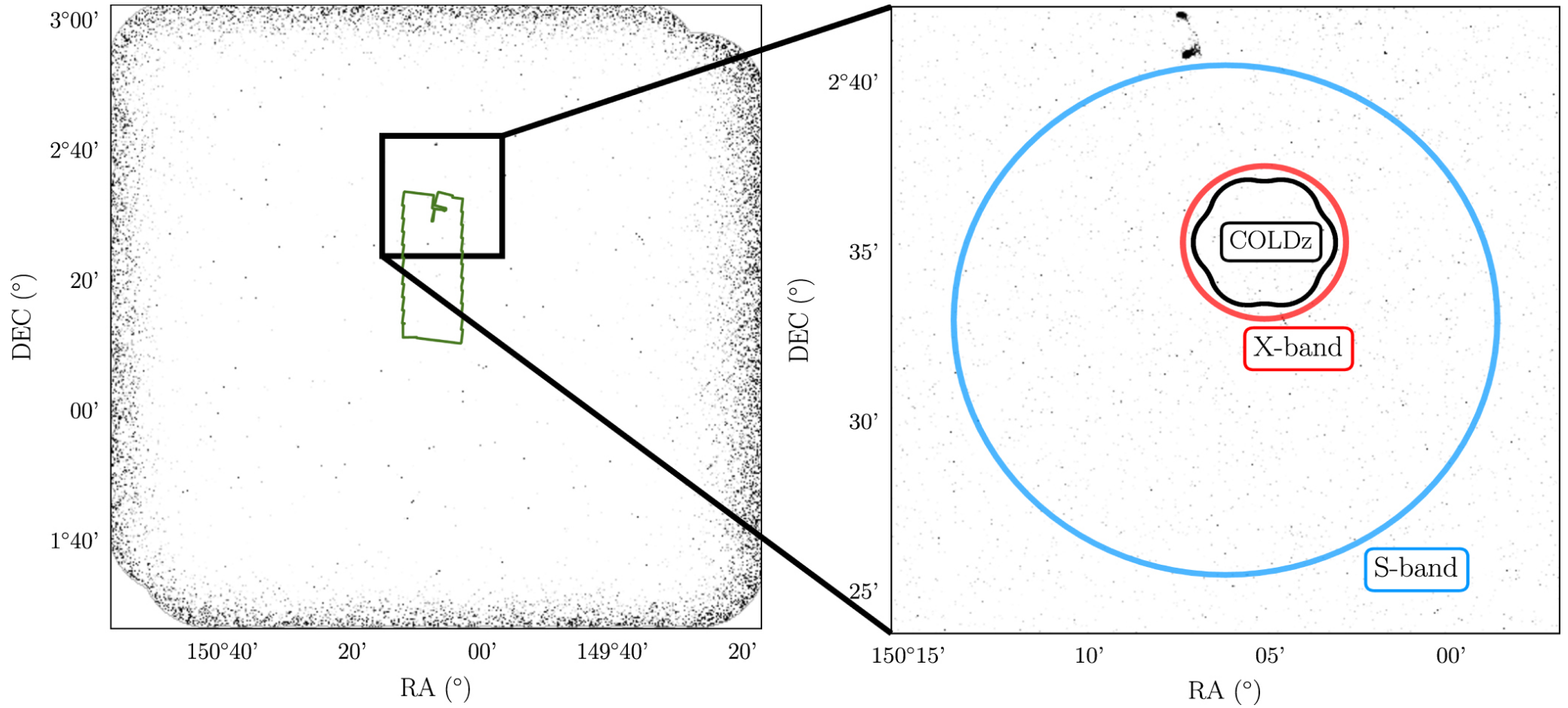
Figure 1. from An Ultradeep Multiband VLA Survey of the Faint Radio Sky (COSMOS-XS): Source Catalog and Number Counts null 2021 APJ 907 5 doi:10.3847/1538-4357/abcaa3 https://dx.doi.org/10.3847/1538-4357/abcaa3 © 2021. The American Astronomical Society. All rights reserved.
