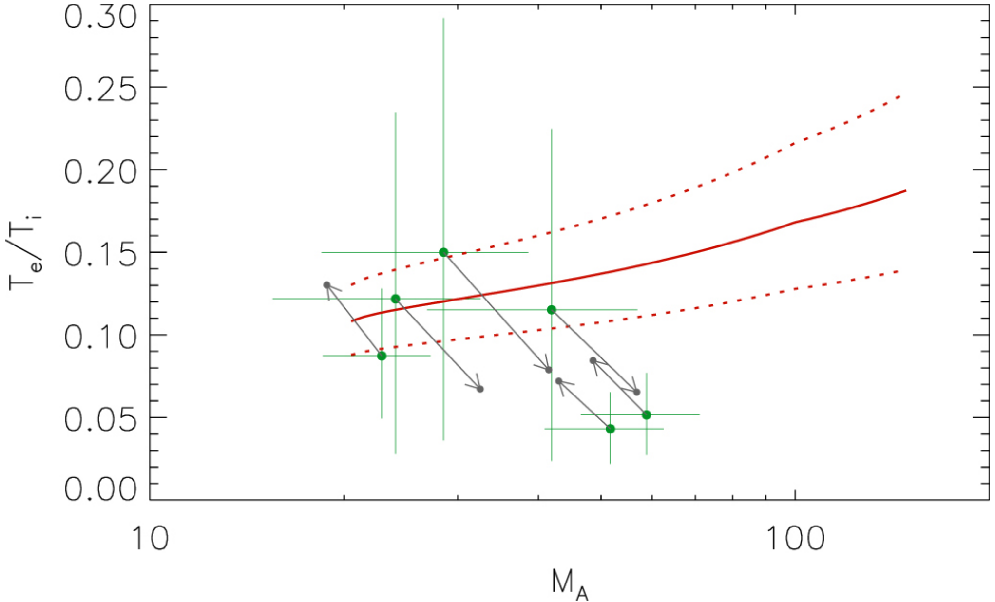
Figure 3. from Kinetic Simulation of Nonrelativistic Perpendicular Shocks of Young Supernova Remnants. IV. Electron Heating null 2020 APJ 904 12 doi:10.3847/1538-4357/abbc19 https://dx.doi.org/10.3847/1538-4357/abbc19 © 2020. The American Astronomical Society. All rights reserved.
