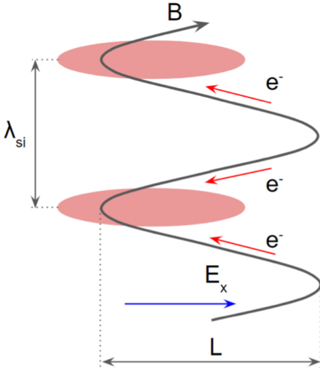
Figure 2. from Kinetic Simulation of Nonrelativistic Perpendicular Shocks of Young Supernova Remnants. IV. Electron Heating null 2020 APJ 904 12 doi:10.3847/1538-4357/abbc19 https://dx.doi.org/10.3847/1538-4357/abbc19 © 2020. The American Astronomical Society. All rights reserved.
