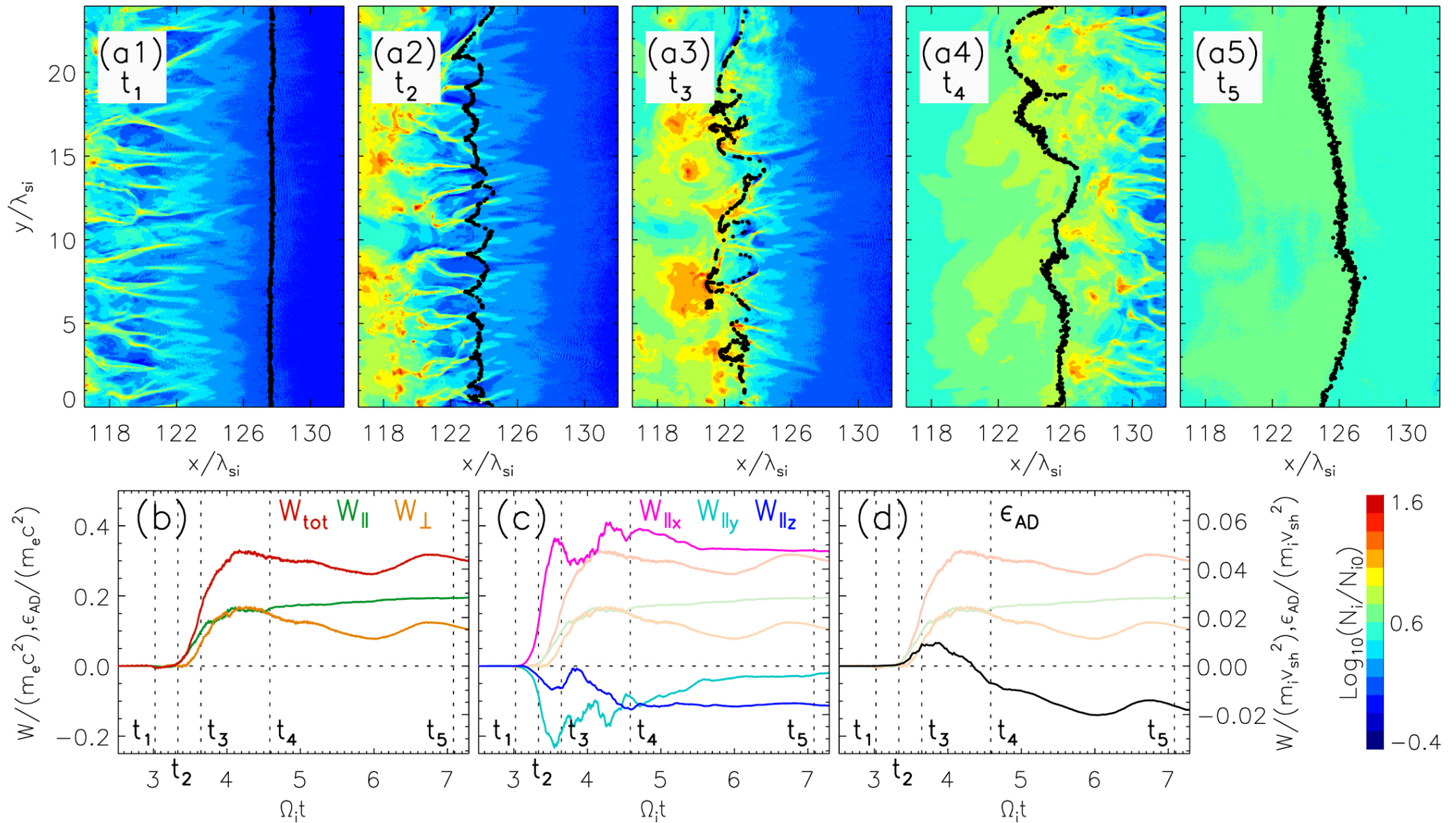
Figure 1. from Kinetic Simulation of Nonrelativistic Perpendicular Shocks of Young Supernova Remnants. IV. Electron Heating null 2020 APJ 904 12 doi:10.3847/1538-4357/abbc19 https://dx.doi.org/10.3847/1538-4357/abbc19 © 2020. The American Astronomical Society. All rights reserved.
