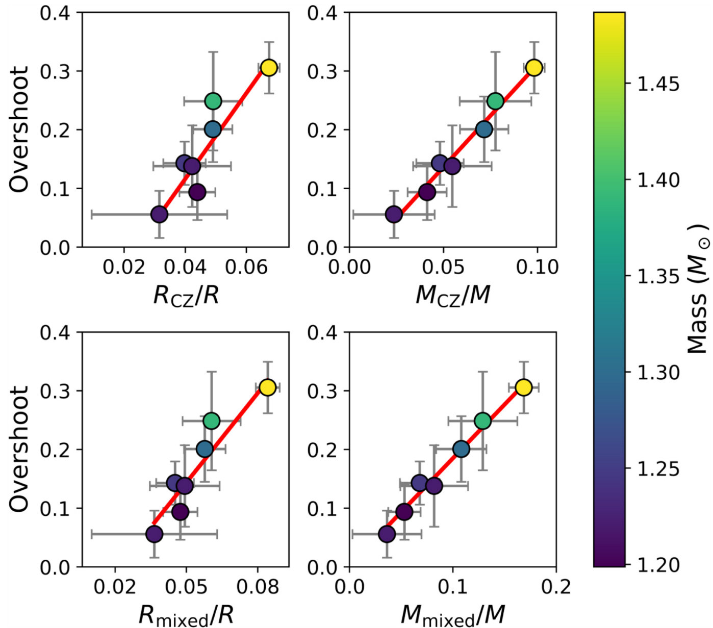
Figure 9. from Examining the Relationship Between Convective Core Overshoot and Stellar Properties Using Asteroseismology null 2020 APJ 904 22 doi:10.3847/1538-4357/abba17 https://dx.doi.org/10.3847/1538-4357/abba17
