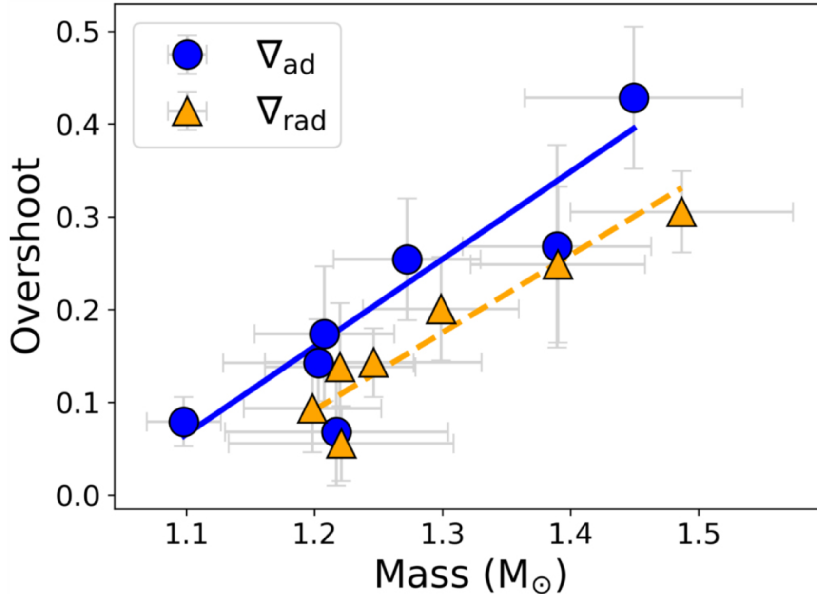
Figure 8. from Examining the Relationship Between Convective Core Overshoot and Stellar Properties Using Asteroseismology null 2020 APJ 904 22 doi:10.3847/1538-4357/abba17 https://dx.doi.org/10.3847/1538-4357/abba17 © 2020. The American Astronomical Society. All rights reserved.
