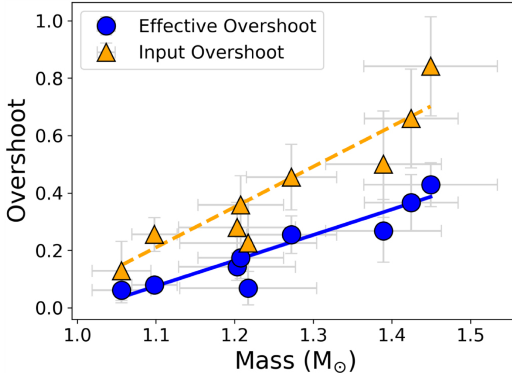
Figure 5. from Examining the Relationship Between Convective Core Overshoot and Stellar Properties Using Asteroseismology null 2020 APJ 904 22 doi:10.3847/1538-4357/abba17 https://dx.doi.org/10.3847/1538-4357/abba17 © 2020. The American Astronomical Society. All rights reserved.
