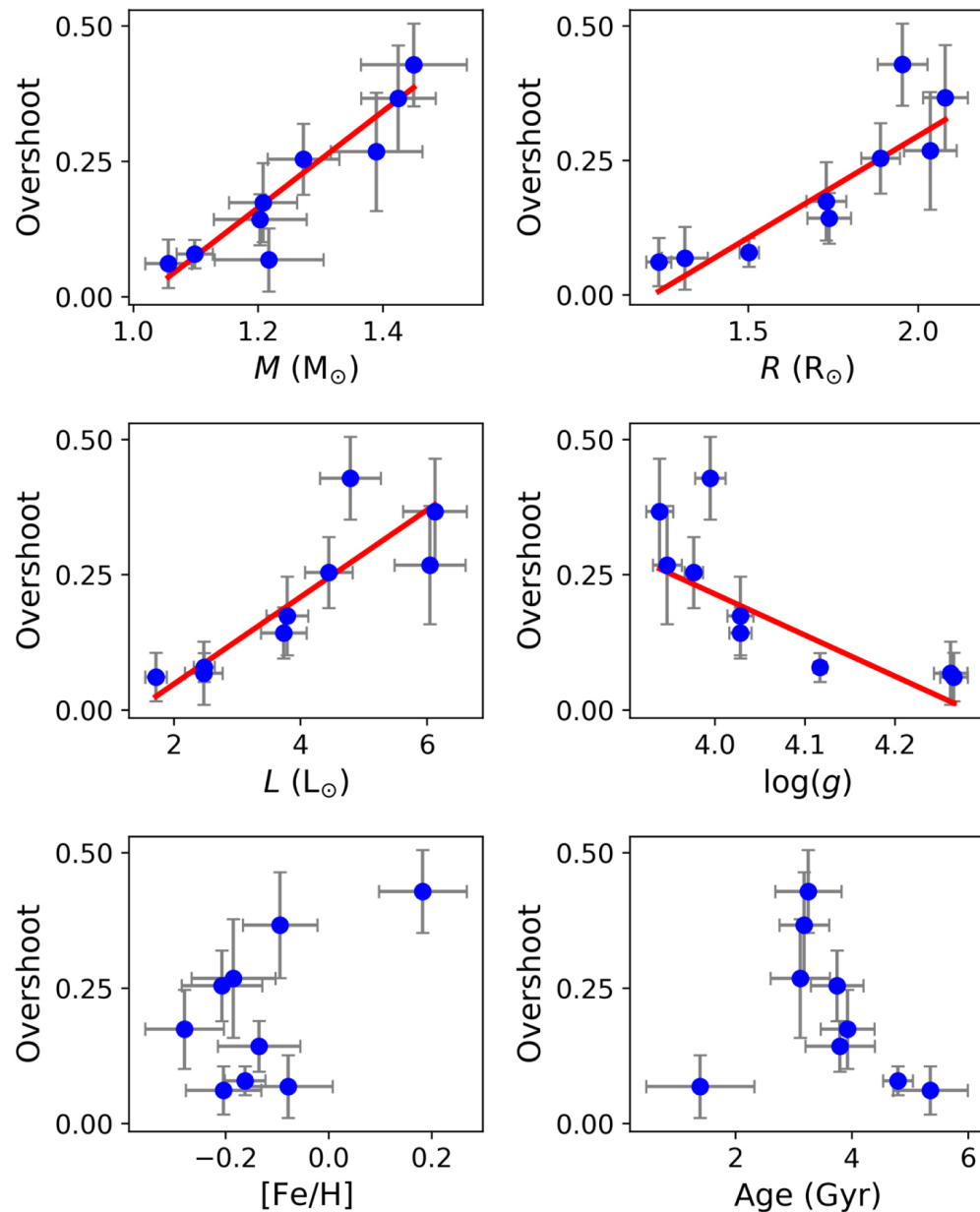
Figure 4. from Examining the Relationship Between Convective Core Overshoot and Stellar Properties Using Asteroseismology null 2020 APJ 904 22 doi:10.3847/1538-4357/abba17 https://dx.doi.org/10.3847/1538-4357/abba17
