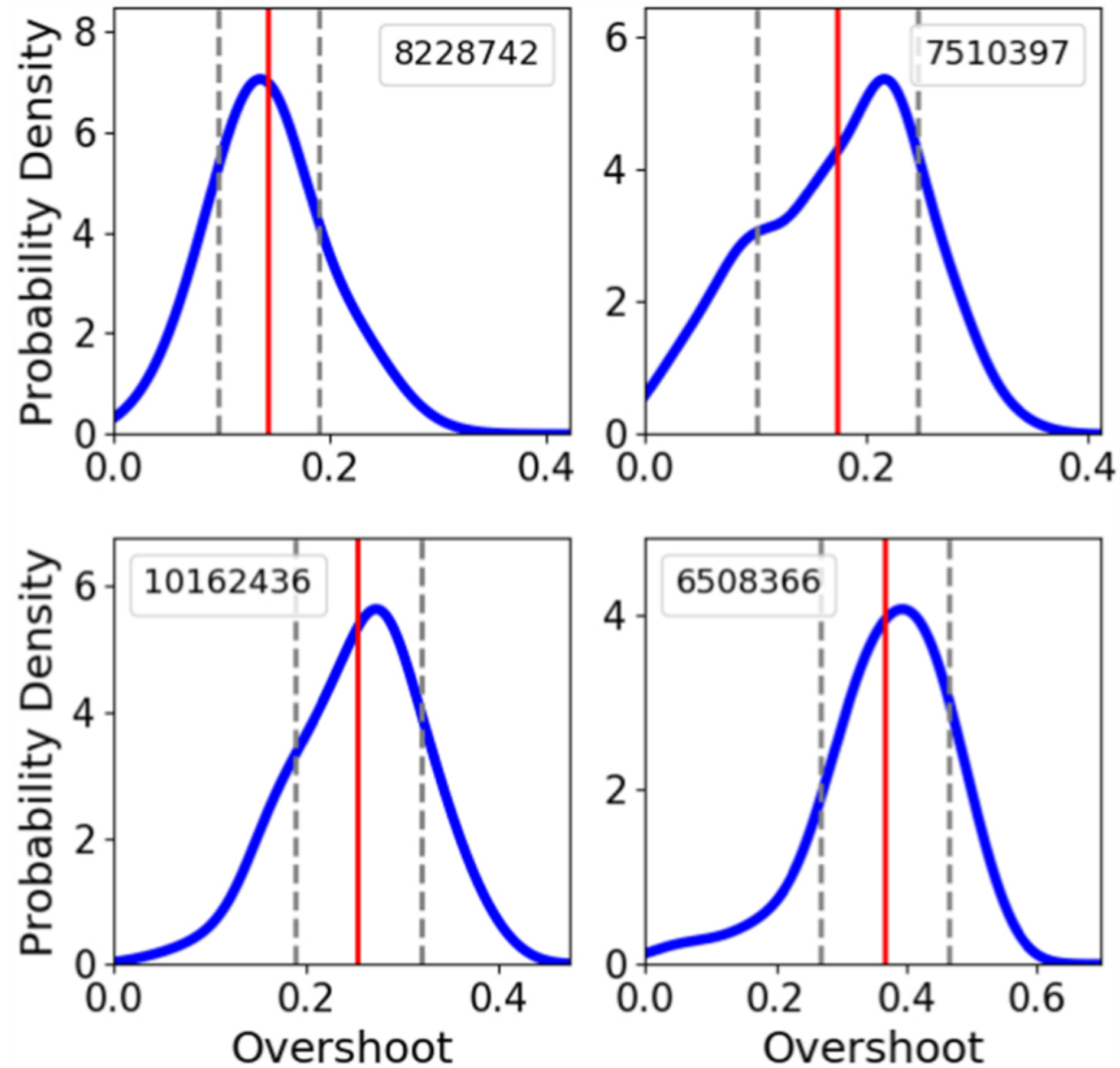
Figure 3. from Examining the Relationship Between Convective Core Overshoot and Stellar Properties Using Asteroseismology null 2020 APJ 904 22 doi:10.3847/1538-4357/abba17 https://dx.doi.org/10.3847/1538-4357/abba17 © 2020. The American Astronomical Society. All rights reserved.
