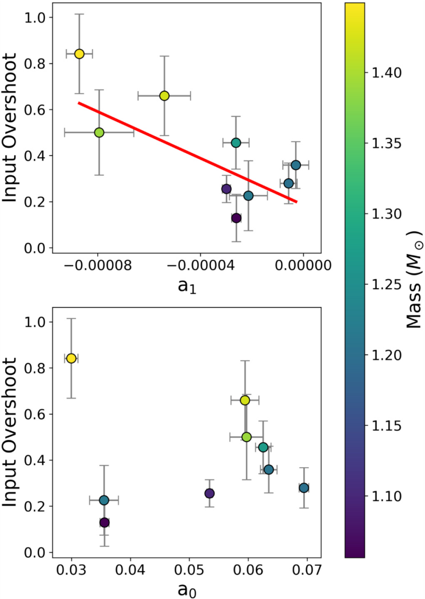
Figure 15. from Examining the Relationship Between Convective Core Overshoot and Stellar Properties Using Asteroseismology null 2020 APJ 904 22 doi:10.3847/1538-4357/abba17 https://dx.doi.org/10.3847/1538-4357/abba17 © 2020. The American Astronomical Society. All rights reserved.
