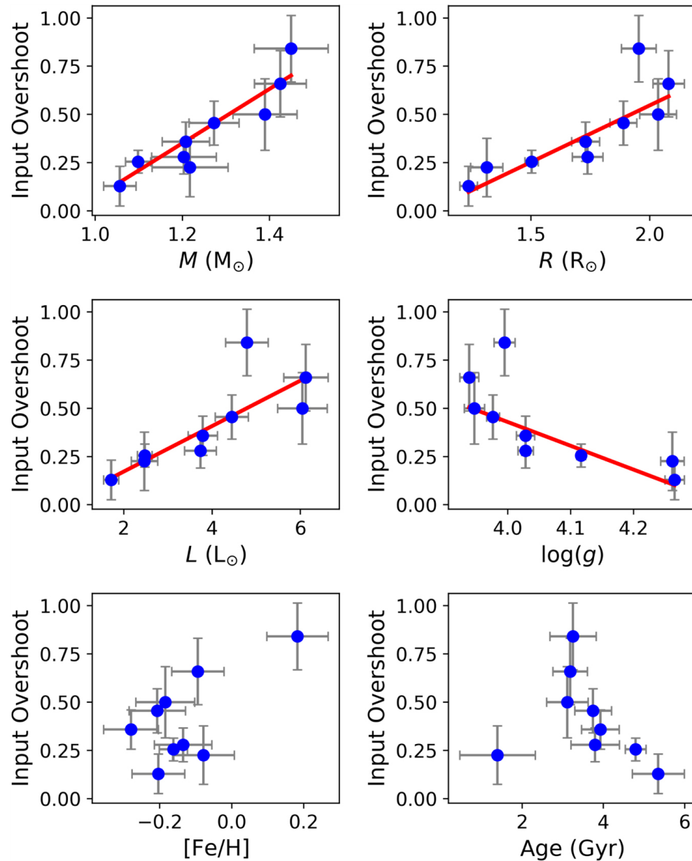
Figure 14. from Examining the Relationship Between Convective Core Overshoot and Stellar Properties Using Asteroseismology null 2020 APJ 904 22 doi:10.3847/1538-4357/abba17 https://dx.doi.org/10.3847/1538-4357/abba17
