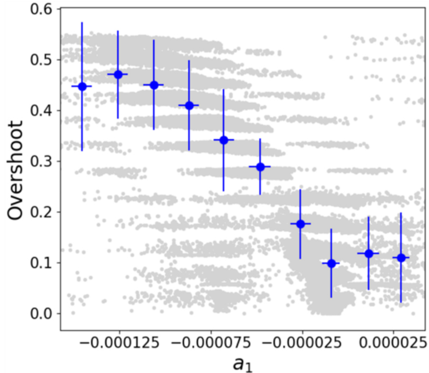
Figure 13. from Examining the Relationship Between Convective Core Overshoot and Stellar Properties Using Asteroseismology null 2020 APJ 904 22 doi:10.3847/1538-4357/abba17 https://dx.doi.org/10.3847/1538-4357/abba17 © 2020. The American Astronomical Society. All rights reserved.
