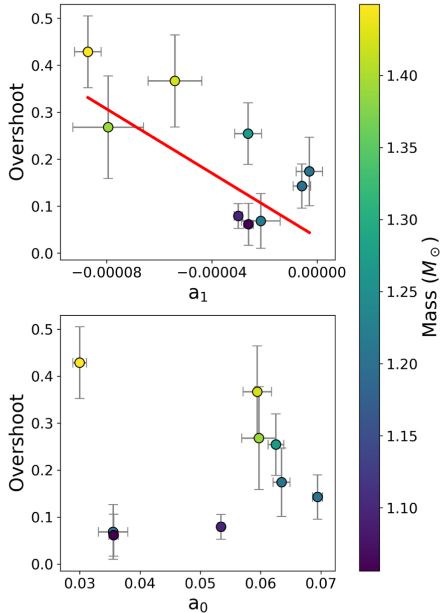
Figure 12. from Examining the Relationship Between Convective Core Overshoot and Stellar Properties Using Asteroseismology null 2020 APJ 904 22 doi:10.3847/1538-4357/abba17 https://dx.doi.org/10.3847/1538-4357/abba17
