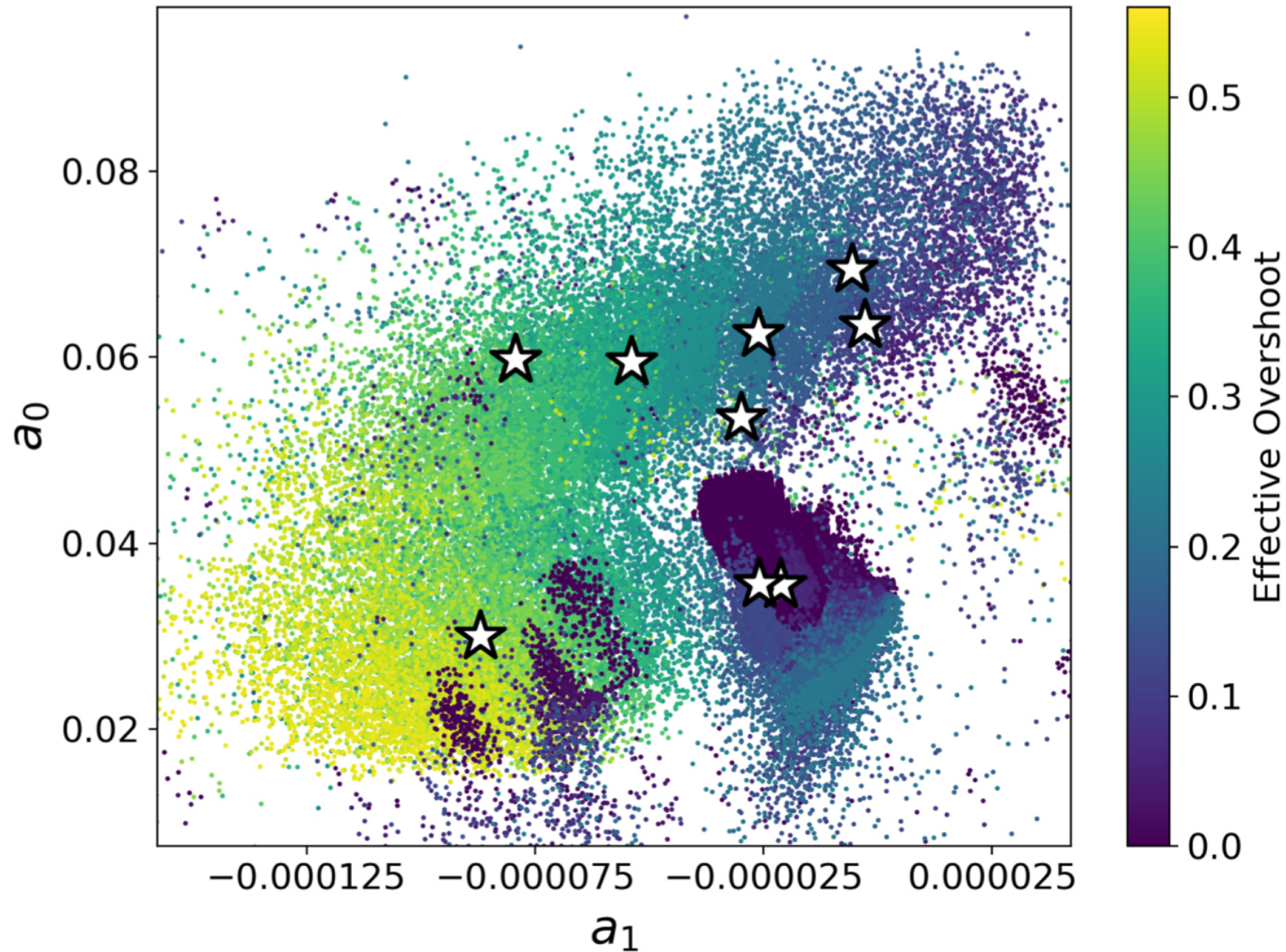
Figure 11. from Examining the Relationship Between Convective Core Overshoot and Stellar Properties Using Asteroseismology null 2020 APJ 904 22 doi:10.3847/1538-4357/abba17 https://dx.doi.org/10.3847/1538-4357/abba17 © 2020. The American Astronomical Society. All rights reserved.
