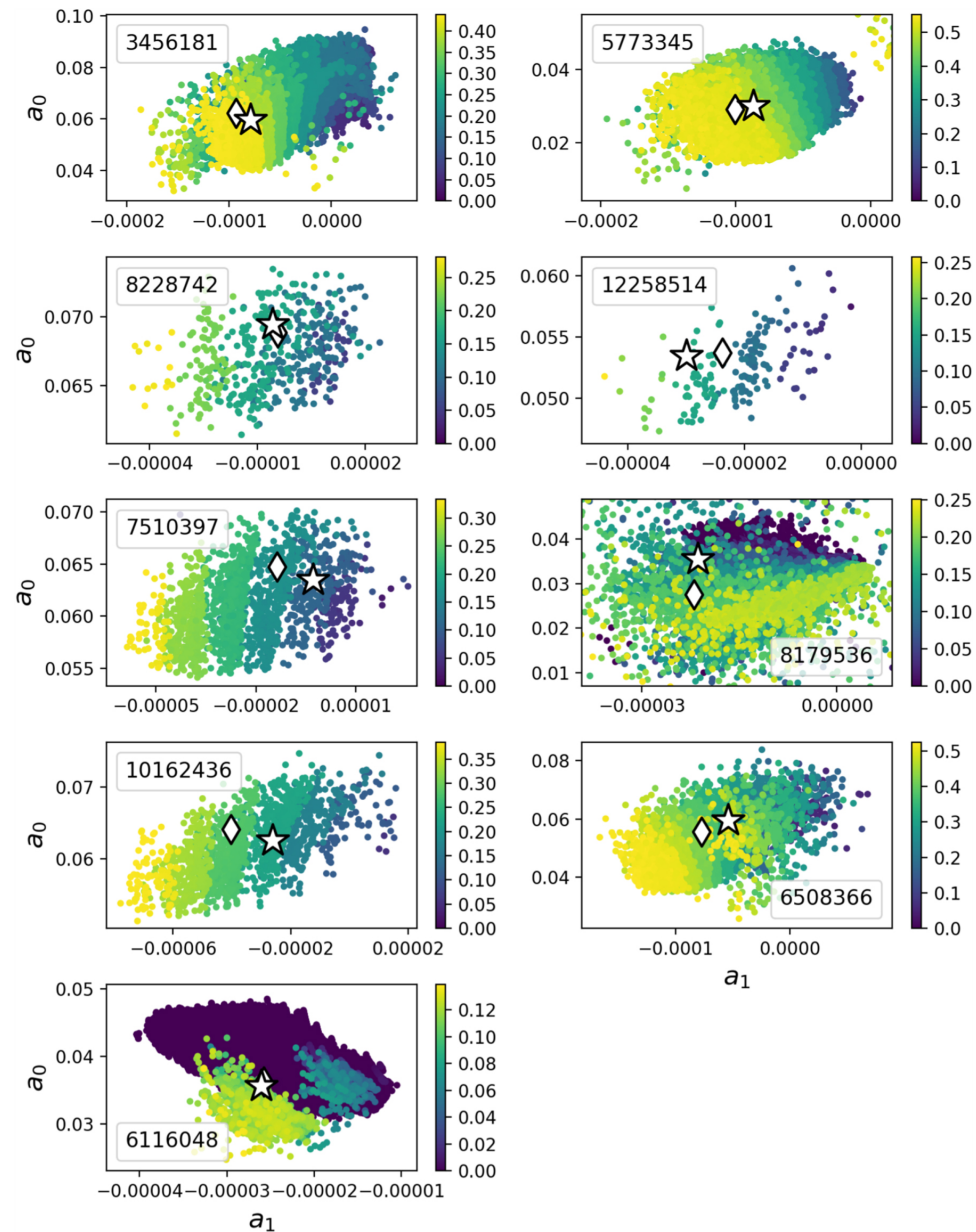
Figure 10. from Examining the Relationship Between Convective Core Overshoot and Stellar Properties Using Asteroseismology null 2020 APJ 904 22 doi:10.3847/1538-4357/abba17 https://dx.doi.org/10.3847/1538-4357/abba17
