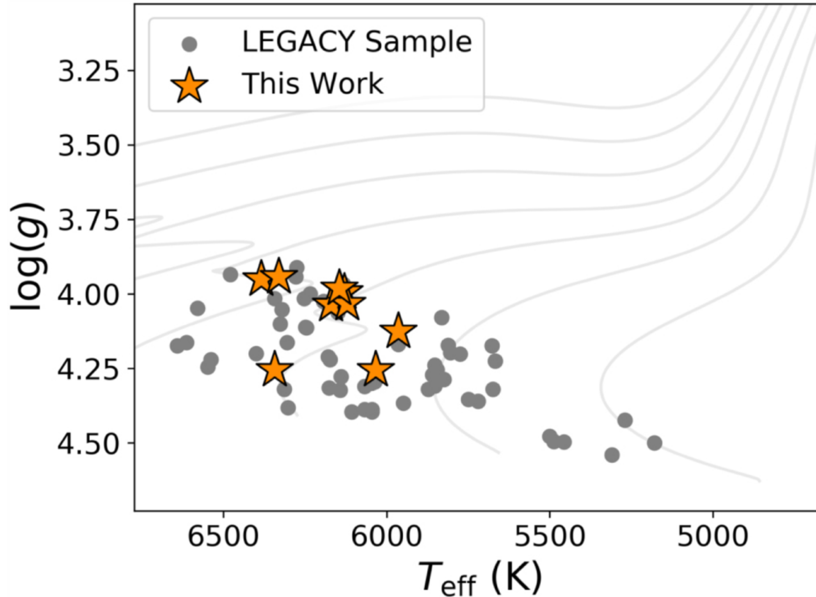
Figure 1. from Examining the Relationship Between Convective Core Overshoot and Stellar Properties Using Asteroseismology null 2020 APJ 904 22 doi:10.3847/1538-4357/abba17 https://dx.doi.org/10.3847/1538-4357/abba17 © 2020. The American Astronomical Society. All rights reserved.
