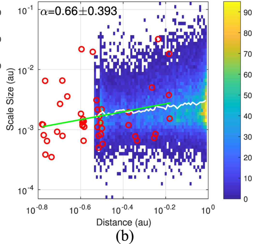
Figure 6. from Small-scale Magnetic Flux Ropes in the First Two Parker Solar Probe Encounters null 2020 APJ 903 76 doi:10.3847/1538-4357/abb820 https://dx.doi.org/10.3847/1538-4357/abb820 © 2020. The American Astronomical Society. All rights reserved.
