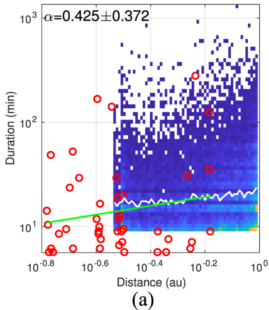
Figure 6. from Small-scale Magnetic Flux Ropes in the First Two Parker Solar Probe Encounters null 2020 APJ 903 76 doi:10.3847/1538-4357/abb820 https://dx.doi.org/10.3847/1538-4357/abb820 © 2020. The American Astronomical Society. All rights reserved.
